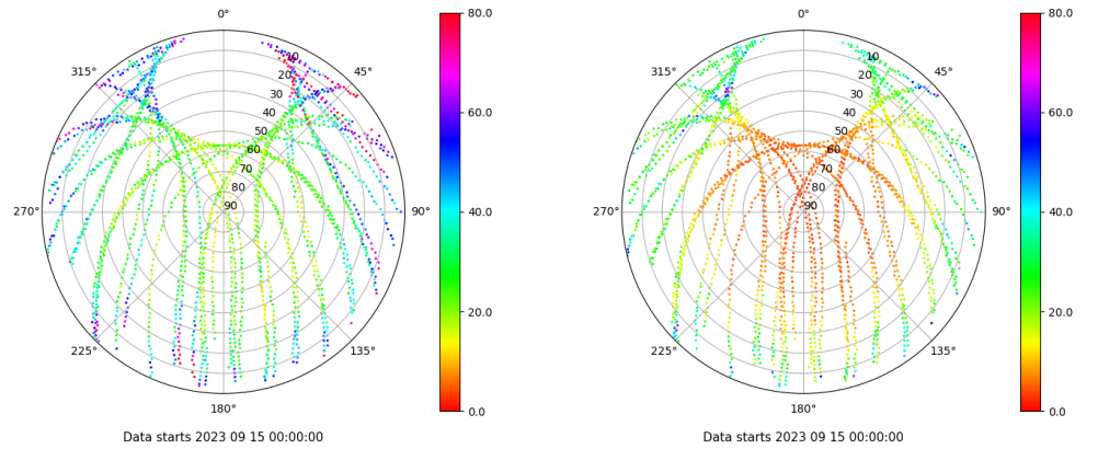
Skyplot for station TALV. Parameter M1C Data file TALV00ESP_R_2023258.xtr Skyplot for station TALV. Parameter M2P Data file TALV00ESP_R_2023258.xtr
