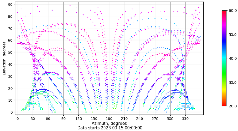
Azimuth-elevation plot for station TALV. Signal to Noise S1C Data file TALV00ESP_R_2023258.xtr
