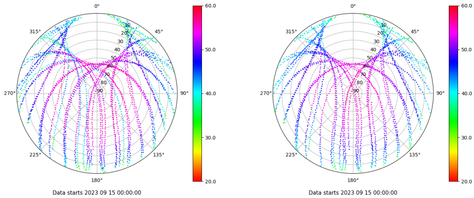
Skyplot for station TALV. Signal to Noise S1C Data file TALV00ESP_R_2023258.xtr Skyplot for station TALV. Signal to Noise S2P Data file TALV00ESP_R_2023258.xtr
