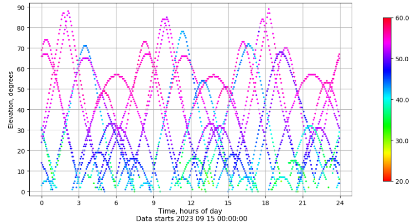
Time-elevation plot for station TALV. Signal to Noise S1C Data file TALV00ESP_R_2023258.xtr
