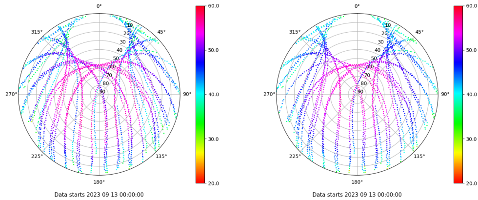
Skyplot for station TALV. Signal to Noise S1C Data file TALV00ESP_R_2023256.xtr Skyplot for station TALV. Signal to Noise S2P Data file TALV00ESP_R_2023256.xtr
