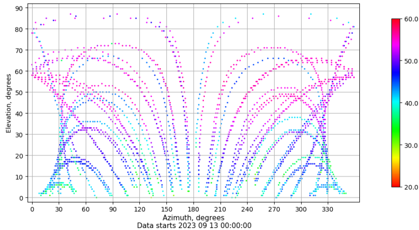
Azimuth-elevation plot for station TALV. Signal to Noise S1C Data file TALV00ESP_R_2023256.xtr
