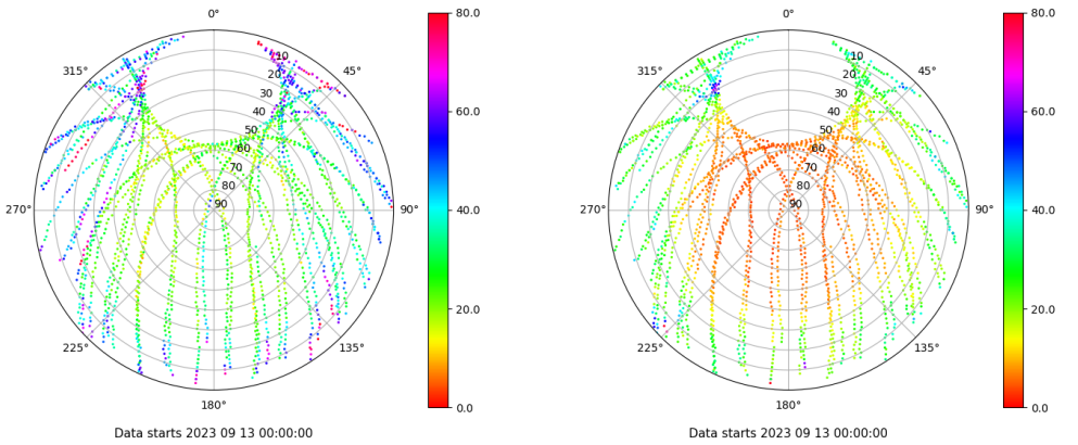
Skyplot for station TALV. Parameter M1C Data file TALV00ESP_R_2023256.xtr Skyplot for station TALV. Parameter M2P Data file TALV00ESP_R_2023256.xtr
