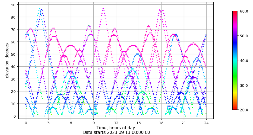
Time-elevation plot for station TALV. Signal to Noise S1C Data file TALV00ESP_R_2023256.xtr
