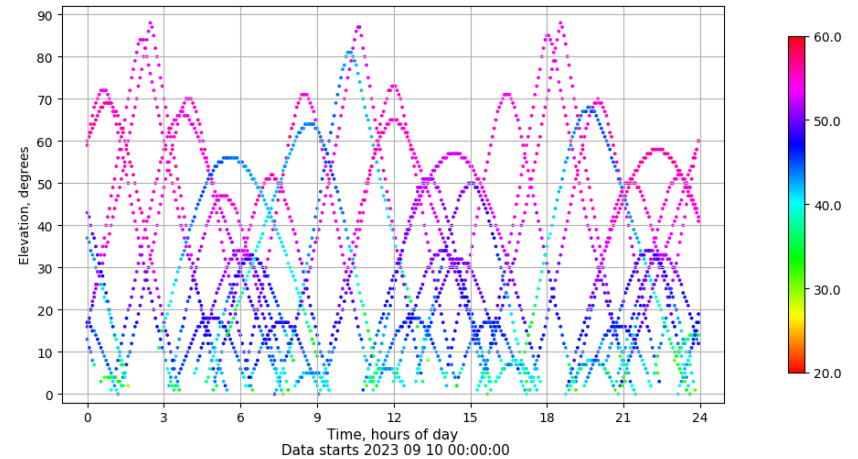
Time-elevation plot for station TALV. Signal to Noise S1C Data file TALV00ESP_R_2023253.xtr
