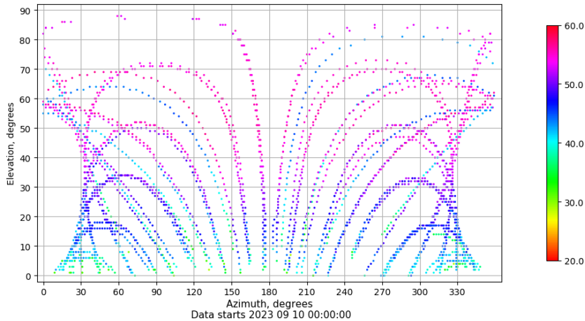
Azimuth-elevation plot for station TALV. Signal to Noise S1C Data file TALV00ESP_R_2023253.xtr
