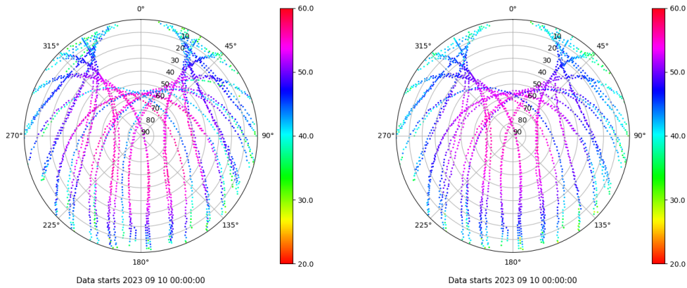
Skyplot for station TALV. Signal to Noise S1C Data file TALV00ESP_R_2023253.xtr Skyplot for station TALV. Signal to Noise S2P Data file TALV00ESP_R_2023253.xtr
