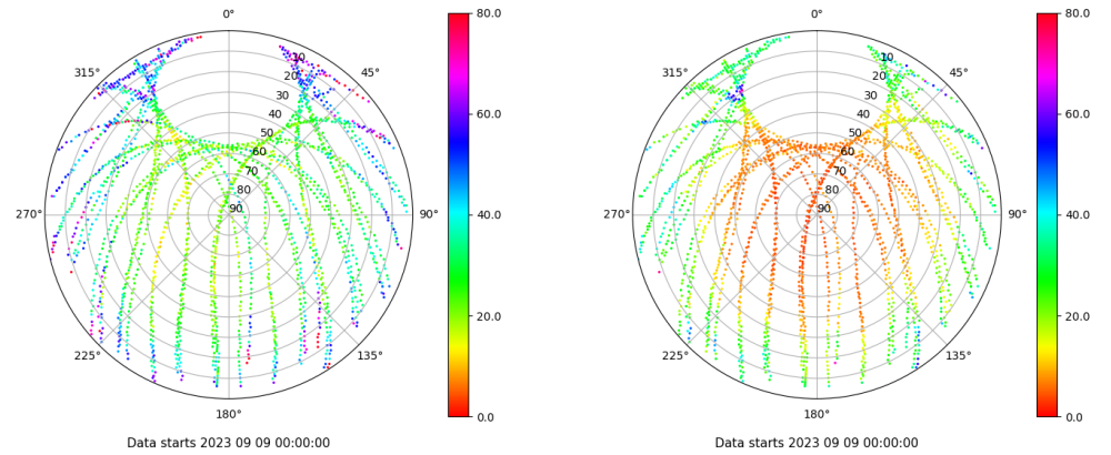
Skyplot for station TALV. Parameter M1C Data file TALV00ESP_R_2023252.xtr Skyplot for station TALV. Parameter M2P Data file TALV00ESP_R_2023252.xtr
