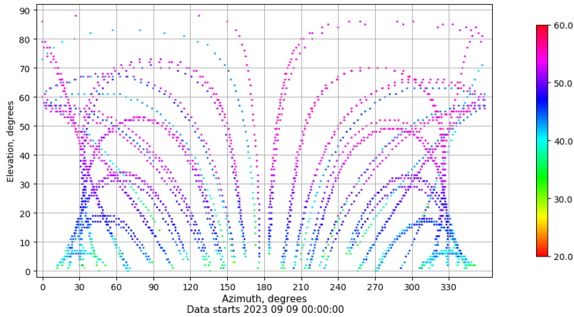
Azimuth-elevation plot for station TALV. Signal to Noise S1C Data file TALV00ESP_R_2023252.xtr
