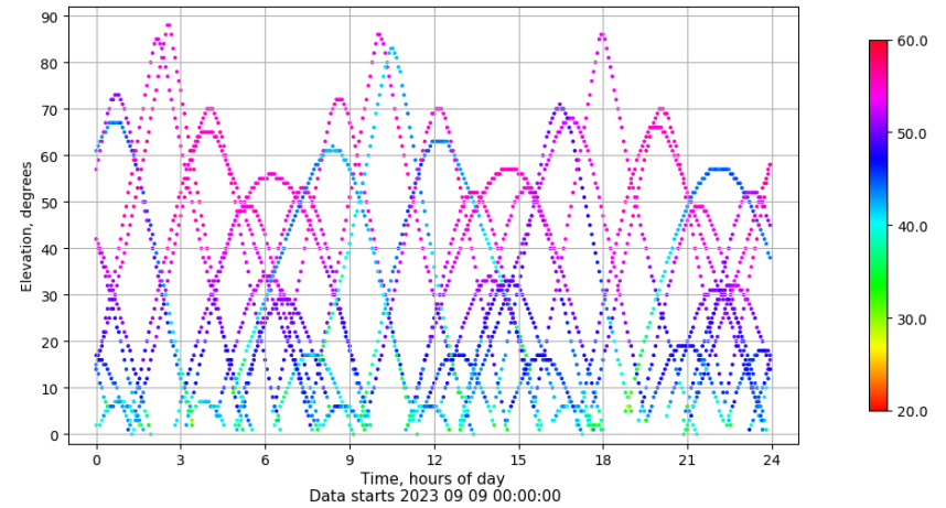
Time-elevation plot for station TALV. Signal to Noise S1C Data file TALV00ESP_R_2023252.xtr
