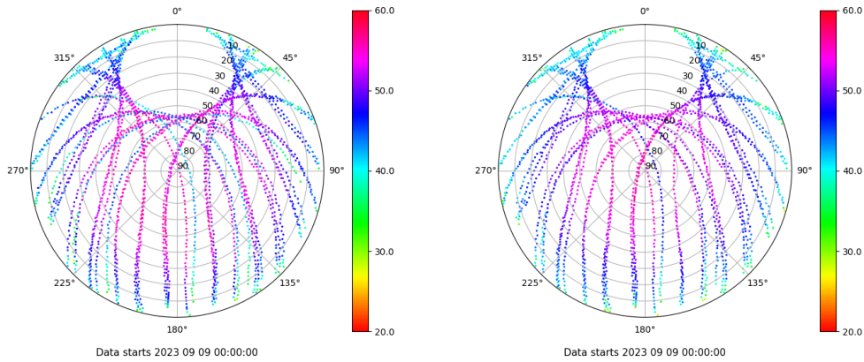
Skyplot for station TALV. Signal to Noise S1C Data file TALV00ESP_R_2023252.xtr Skyplot for station TALV. Signal to Noise S2P Data file TALV00ESP_R_2023252.xtr
