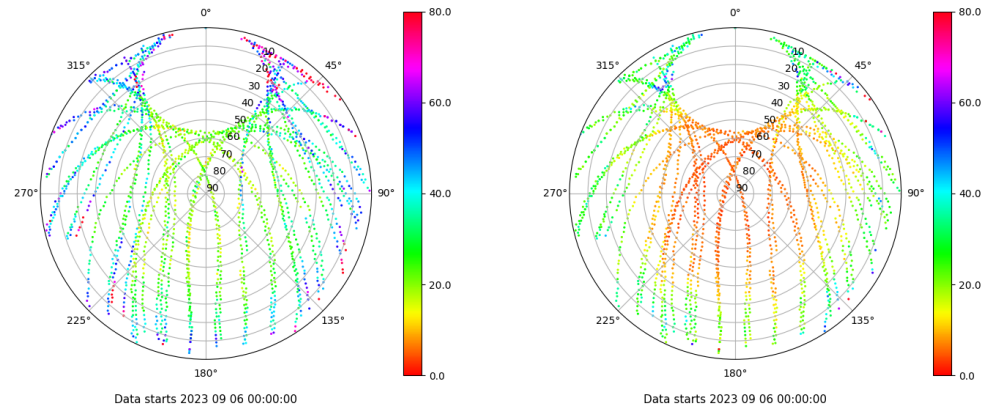
Skyplot for station TALV. Parameter M1C Data file TALV00ESP_R_2023249.xtr Skyplot for station TALV. Parameter M2P Data file TALV00ESP_R_2023249.xtr
