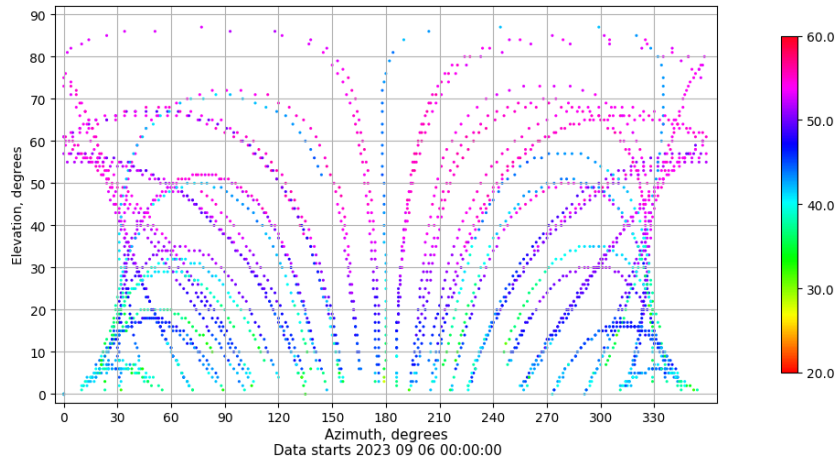
Azimuth-elevation plot for station TALV. Signal to Noise S1C Data file TALV00ESP_R_2023249.xtr
