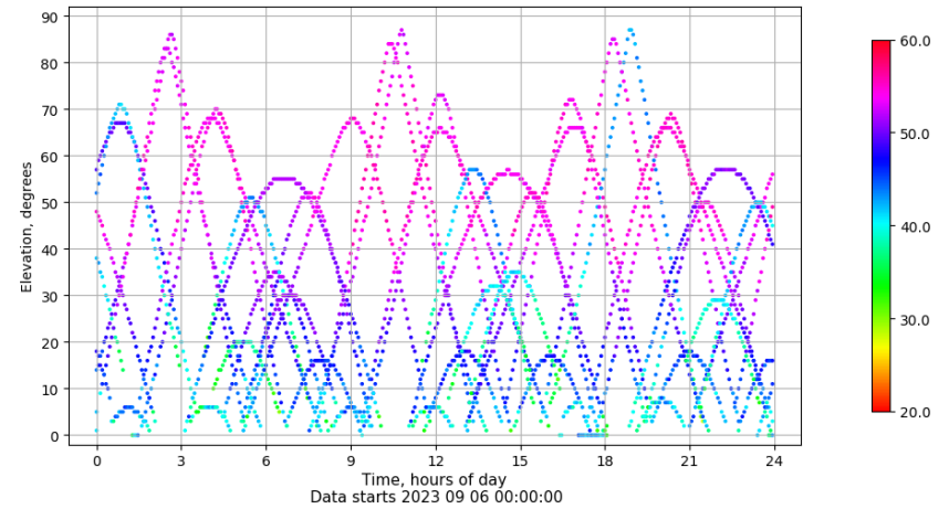
Time-elevation plot for station TALV. Signal to Noise S1C Data file TALV00ESP_R_2023249.xtr
