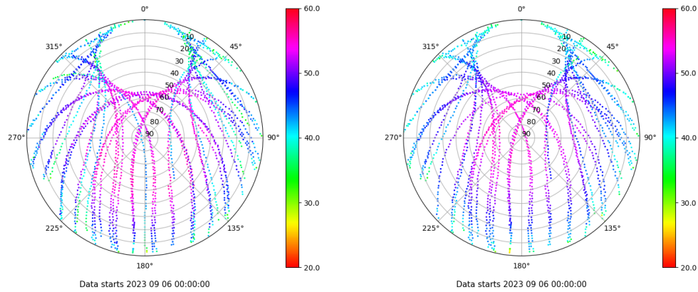
Skyplot for station TALV. Signal to Noise S1C Data file TALV00ESP_R_2023249.xtr Skyplot for station TALV. Signal to Noise S2P Data file TALV00ESP_R_2023249.xtr
