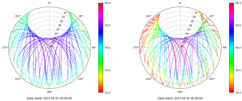
Skyplot for station TALV. Signal to Noise S1C Data file TALV00ESP_R_2023248.xtr Skyplot for station TALV. Signal to Noise S2W Data file TALV00ESP_R_2023248.xtr
