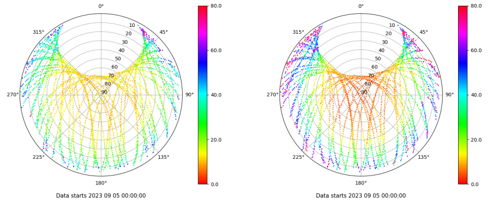
Skyplot for station TALV. Parameter M1C Data file TALV00ESP_R_2023248.xtr Skyplot for station TALV. Parameter M2W Data file TALV00ESP_R_2023248.xtr
