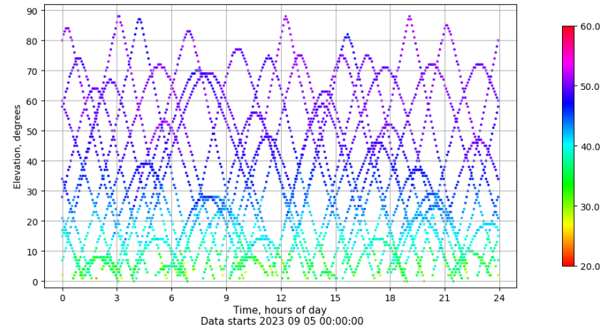
Time-elevation plot for station TALV. Signal to Noise S1C Data file TALV00ESP_R_2023248.xtr
