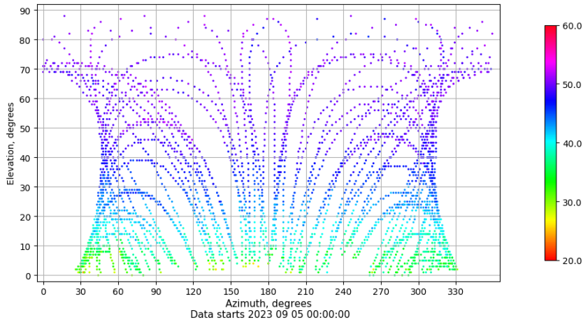
Azimuth-elevation plot for station TALV. Signal to Noise S1C Data file TALV00ESP_R_2023248.xtr
