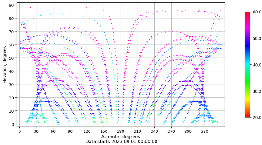
Azimuth-elevation plot for station TALV. Signal to Noise S1C Data file TALV00ESP_R_2023244.xtr
