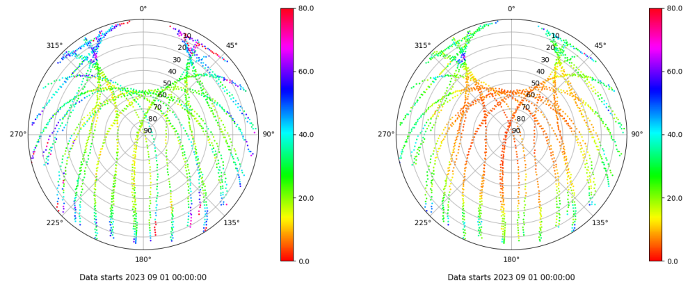
Skyplot for station TALV. Parameter M1C Data file TALV00ESP_R_2023244.xtr Skyplot for station TALV. Parameter M2P Data file TALV00ESP_R_2023244.xtr
