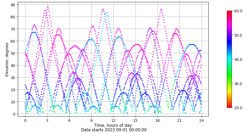
Time-elevation plot for station TALV. Signal to Noise S1C Data file TALV00ESP_R_2023244.xtr
