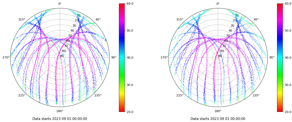
Skyplot for station TALV. Signal to Noise S1C Data file TALV00ESP_R_2023244.xtr Skyplot for station TALV. Signal to Noise S2P Data file TALV00ESP_R_2023244.xtr
