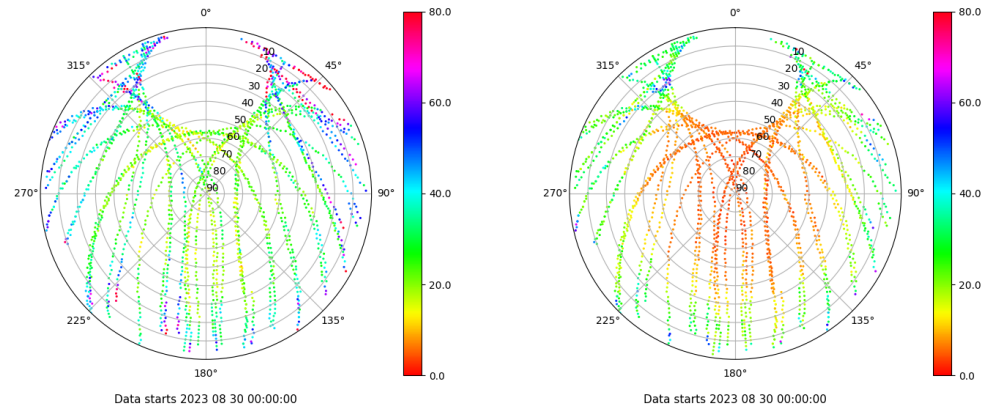
Skyplot for station TALV. Parameter M1C Data file TALV00ESP_R_2023242.xtr Skyplot for station TALV. Parameter M2P Data file TALV00ESP_R_2023242.xtr
