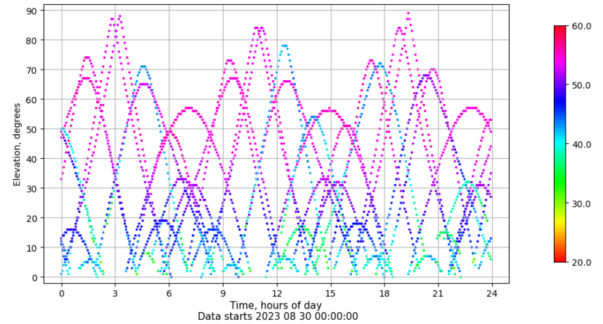
Time-elevation plot for station TALV. Signal to Noise S1C Data file TALV00ESP_R_2023242.xtr
