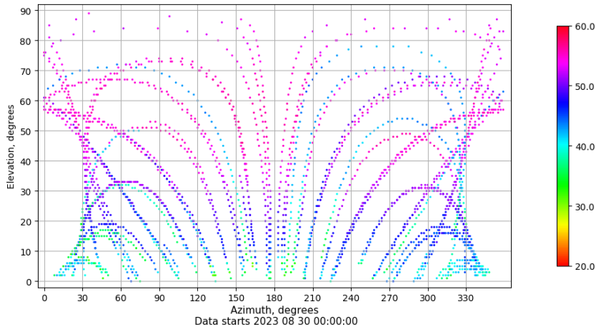
Azimuth-elevation plot for station TALV. Signal to Noise S1C Data file TALV00ESP_R_2023242.xtr
