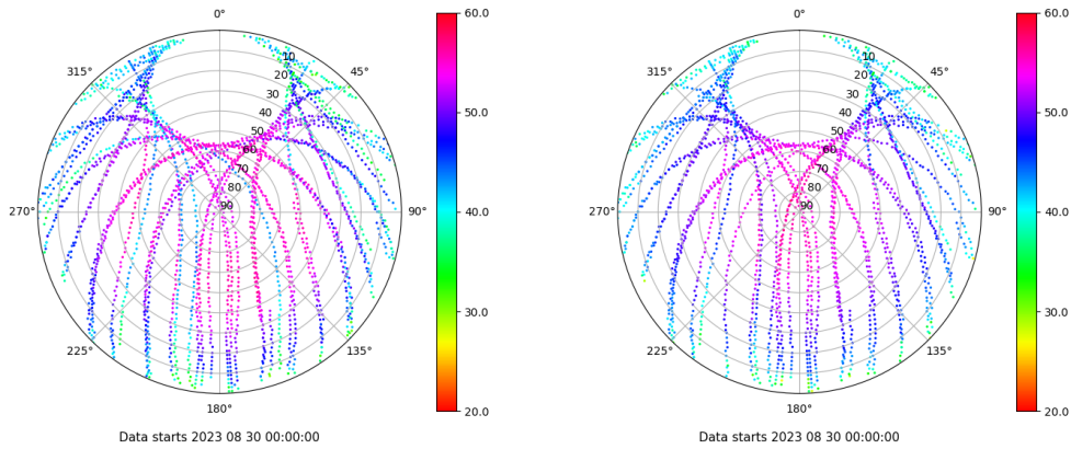
Skyplot for station TALV. Signal to Noise S1C Data file TALV00ESP_R_2023242.xtr Skyplot for station TALV. Signal to Noise S2P Data file TALV00ESP_R_2023242.xtr
