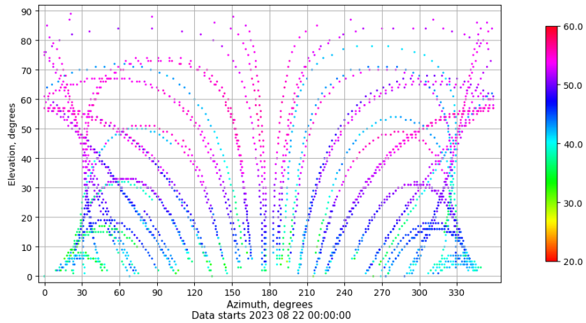
Azimuth-elevation plot for station TALV. Signal to Noise S1C Data file TALV00ESP_R_2023234.xtr
