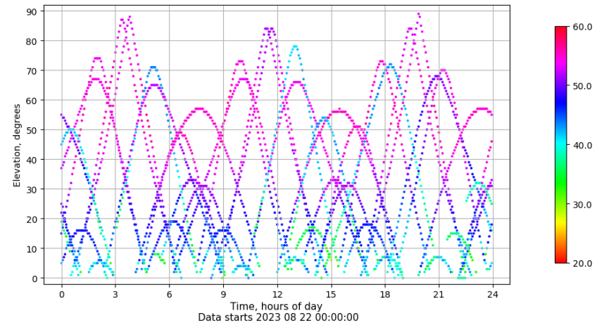
Time-elevation plot for station TALV. Signal to Noise S1C Data file TALV00ESP_R_2023234.xtr
