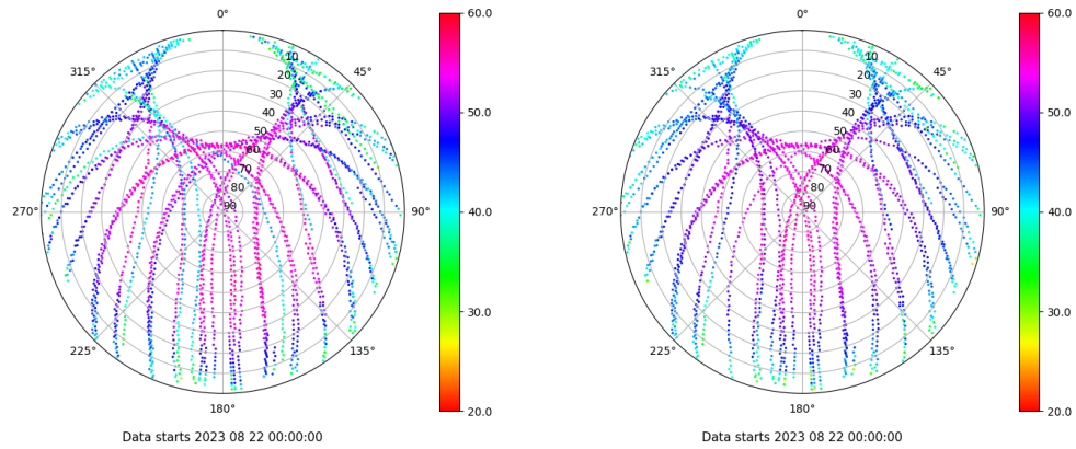
Skyplot for station TALV. Signal to Noise S1C Data file TALV00ESP_R_2023234.xtr Skyplot for station TALV. Signal to Noise S2P Data file TALV00ESP_R_2023234.xtr
