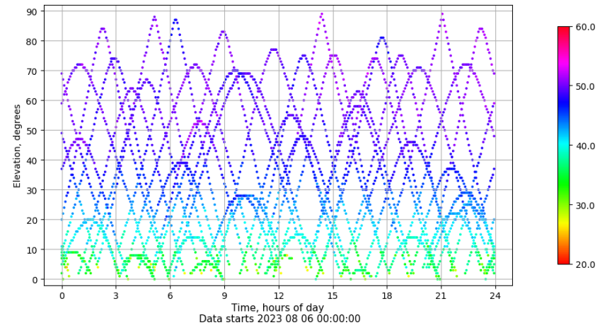
Time-elevation plot for station TALV. Signal to Noise S1C Data file TALV00ESP_R_2023218.xtr
