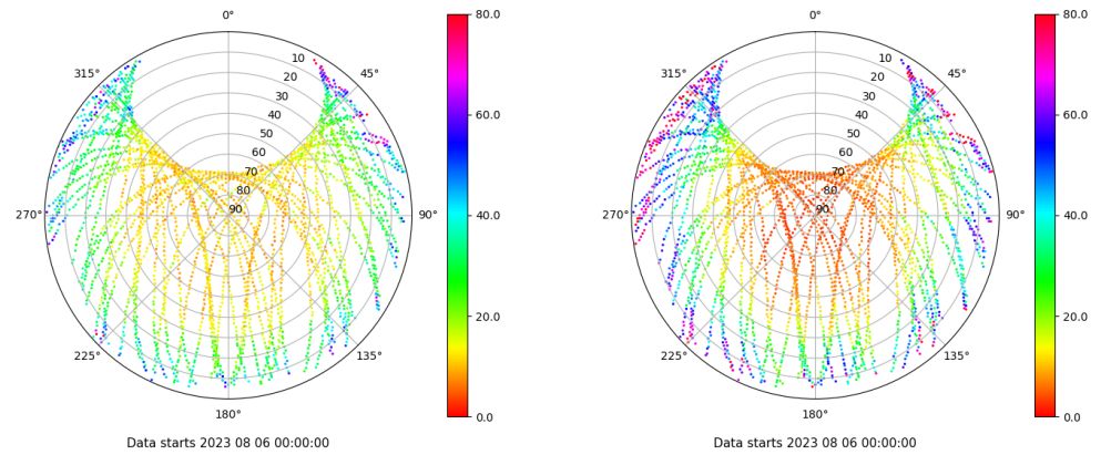
Skyplot for station TALV. Parameter M1C Data file TALV00ESP_R_2023218.xtr Skyplot for station TALV. Parameter M2W Data file TALV00ESP_R_2023218.xtr
