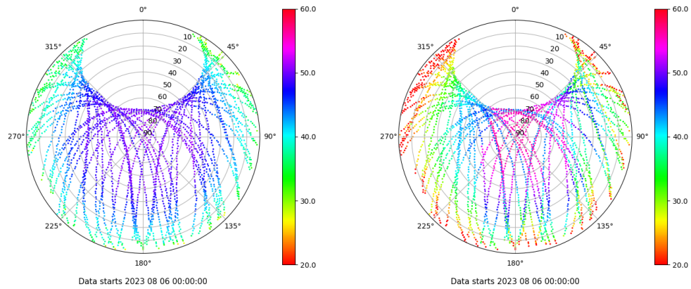
Skyplot for station TALV. Signal to Noise S1C Data file TALV00ESP_R_2023218.xtr Skyplot for station TALV. Signal to Noise S2W Data file TALV00ESP_R_2023218.xtr
