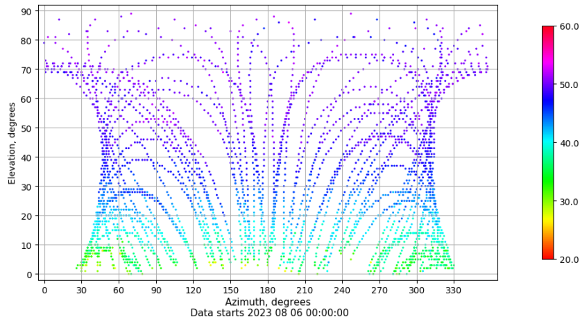
Azimuth-elevation plot for station TALV. Signal to Noise S1C Data file TALV00ESP_R_2023218.xtr
