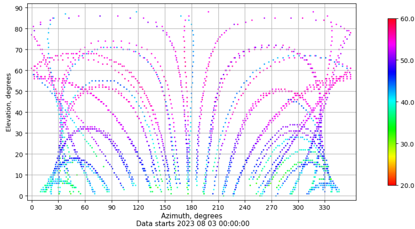
Azimuth-elevation plot for station TALV. Signal to Noise S1C Data file TALV00ESP_R_2023215.xtr
