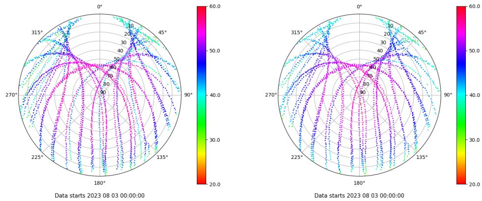
Skyplot for station TALV. Signal to Noise S1C Data file TALV00ESP_R_2023215.xtr Skyplot for station TALV. Signal to Noise S2P Data file TALV00ESP_R_2023215.xtr
