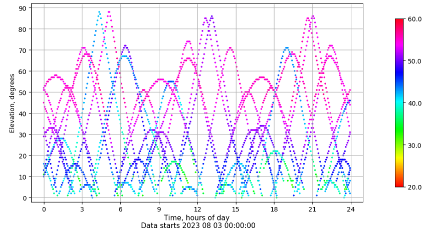
Time-elevation plot for station TALV. Signal to Noise S1C Data file TALV00ESP_R_2023215.xtr
