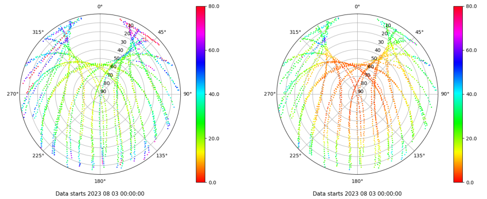
Skyplot for station TALV. Parameter M1C Data file TALV00ESP_R_2023215.xtr Skyplot for station TALV. Parameter M2P Data file TALV00ESP_R_2023215.xtr
