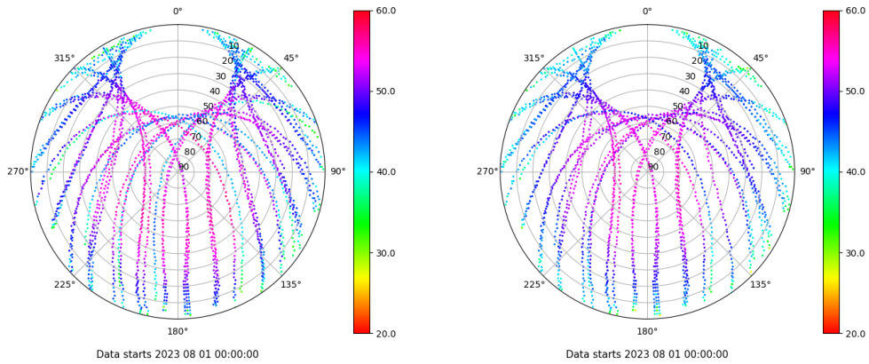
Skyplot for station TALV. Signal to Noise S1C Data file TALV00ESP_R_2023213.xtr Skyplot for station TALV. Signal to Noise S2P Data file TALV00ESP_R_2023213.xtr
