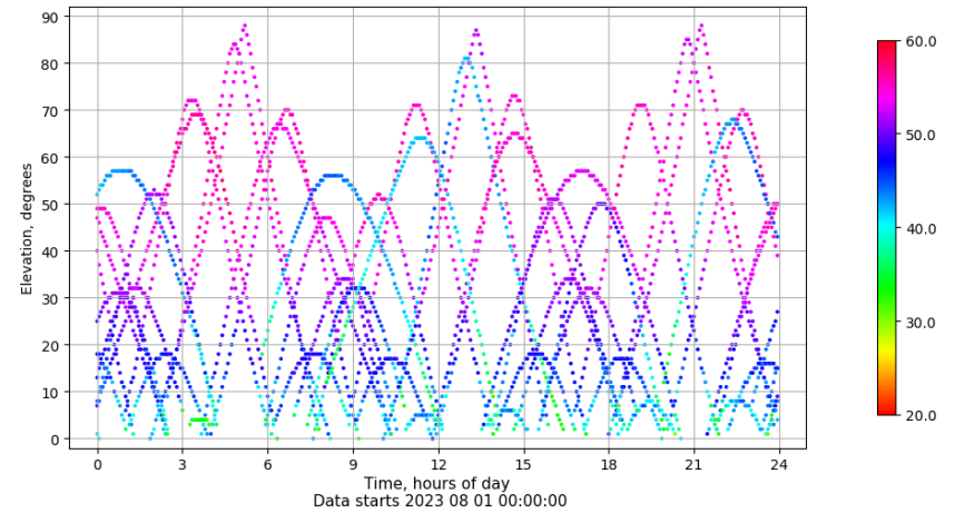
Time-elevation plot for station TALV. Signal to Noise S1C Data file TALV00ESP_R_2023213.xtr
