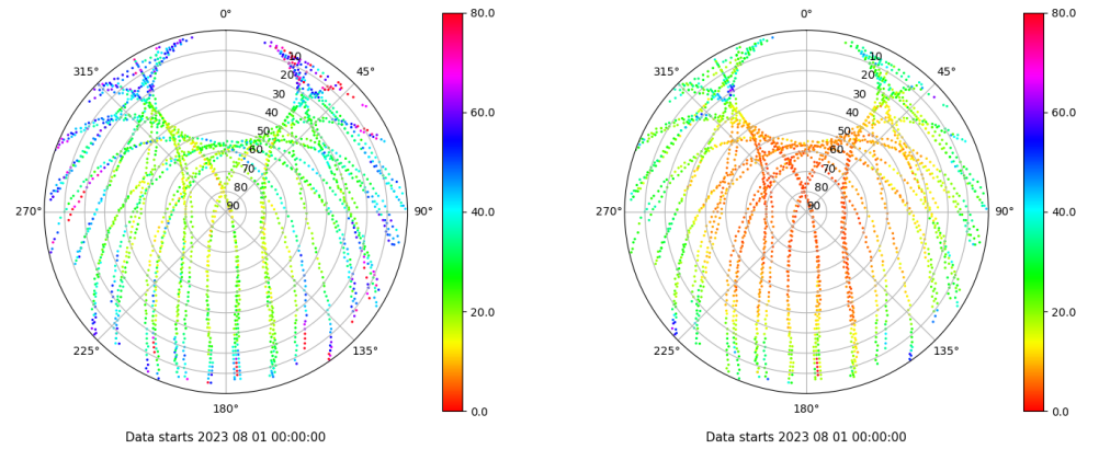
Skyplot for station TALV. Parameter M1C Data file TALV00ESP_R_2023213.xtr Skyplot for station TALV. Parameter M2P Data file TALV00ESP_R_2023213.xtr
