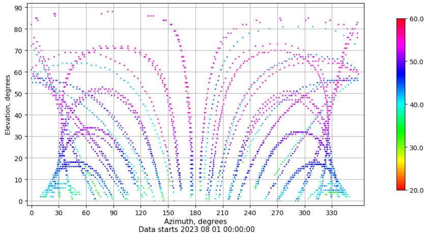
Azimuth-elevation plot for station TALV. Signal to Noise S1C Data file TALV00ESP_R_2023213.xtr
