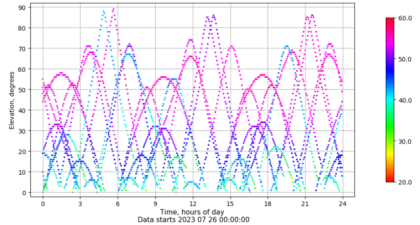
Time-elevation plot for station TALV. Signal to Noise S1C Data file TALV00ESP_R_2023207.xtr
