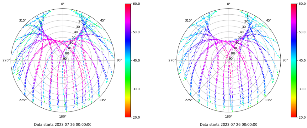
Skyplot for station TALV. Signal to Noise S1C Data file TALV00ESP_R_2023207.xtr Skyplot for station TALV. Signal to Noise S2P Data file TALV00ESP_R_2023207.xtr
