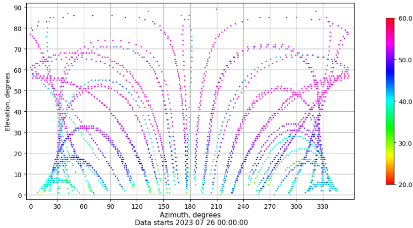
Azimuth-elevation plot for station TALV. Signal to Noise S1C Data file TALV00ESP_R_2023207.xtr
