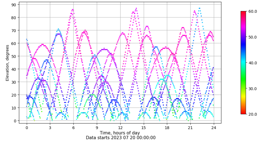
Time-elevation plot for station TALV. Signal to Noise S1C Data file TALV00ESP_R_2023201.xtr
