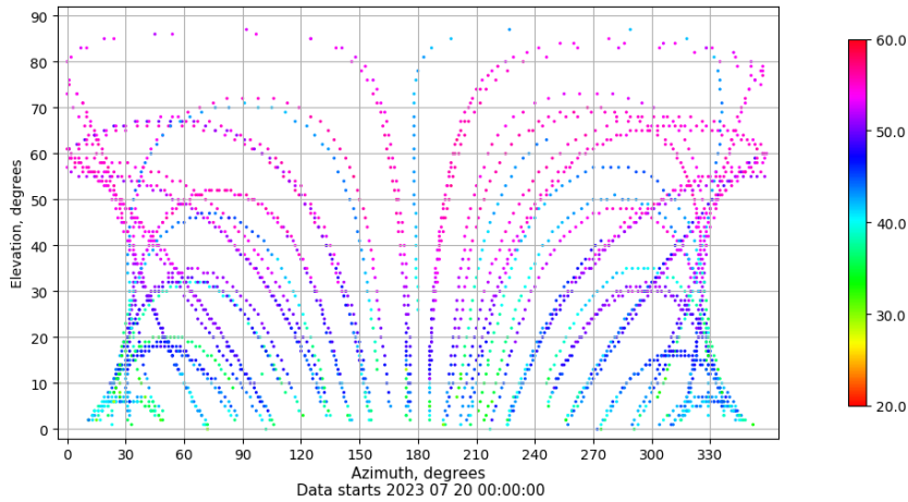
Azimuth-elevation plot for station TALV. Signal to Noise S1C Data file TALV00ESP_R_2023201.xtr
