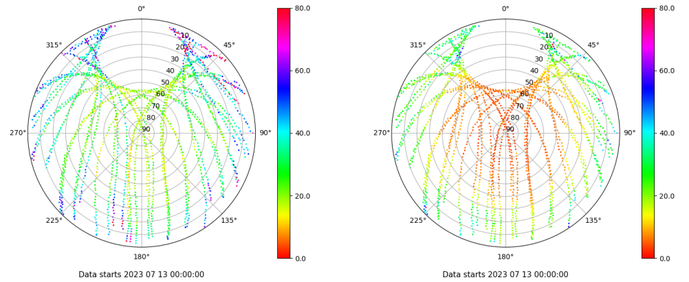
Skyplot for station TALV. Parameter M1C Data file TALV00ESP_R_2023194.xtr Skyplot for station TALV. Parameter M2P Data file TALV00ESP_R_2023194.xtr
