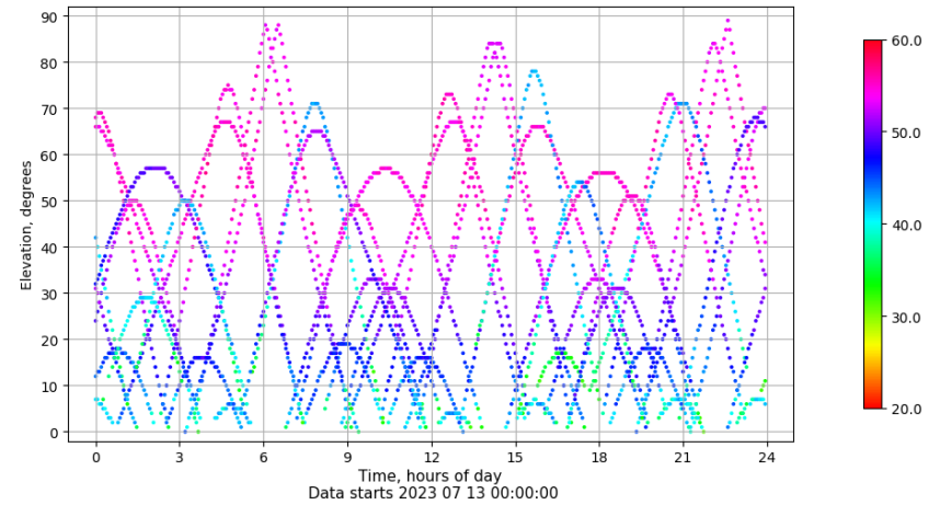
Time-elevation plot for station TALV. Signal to Noise S1C Data file TALV00ESP_R_2023194.xtr
