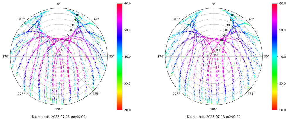
Skyplot for station TALV. Signal to Noise S1C Data file TALV00ESP_R_2023194.xtr Skyplot for station TALV. Signal to Noise S2P Data file TALV00ESP_R_2023194.xtr
