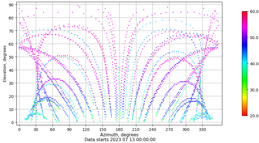
Azimuth-elevation plot for station TALV. Signal to Noise S1C Data file TALV00ESP_R_2023194.xtr
