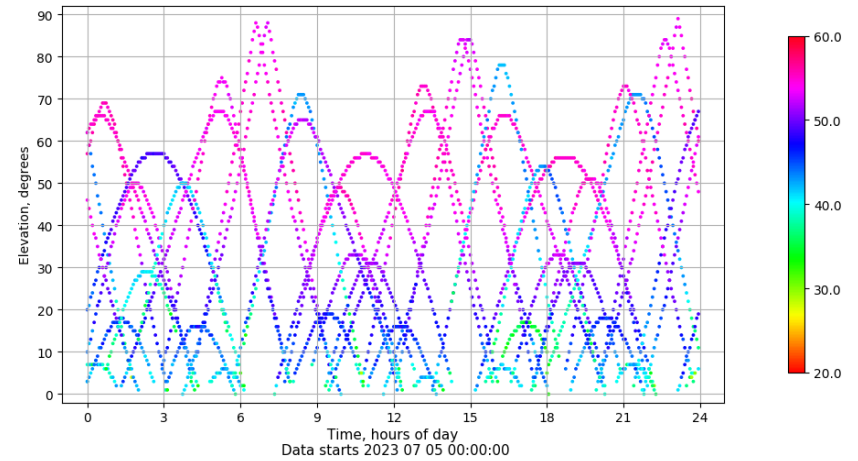
Time-elevation plot for station TALV. Signal to Noise S1C Data file TALV00ESP_R_2023186.xtr
