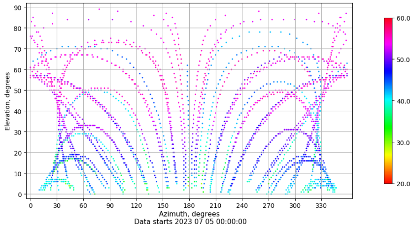
Azimuth-elevation plot for station TALV. Signal to Noise S1C Data file TALV00ESP_R_2023186.xtr
