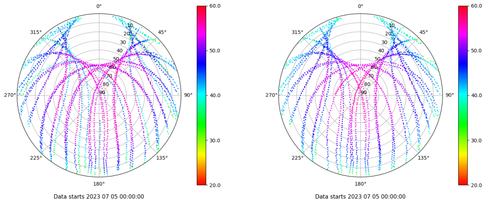
Skyplot for station TALV. Signal to Noise S1C Data file TALV00ESP_R_2023186.xtr Skyplot for station TALV. Signal to Noise S2P Data file TALV00ESP_R_2023186.xtr
