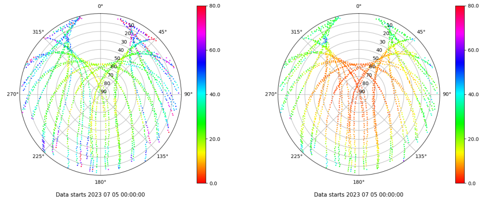
Skyplot for station TALV. Parameter M1C Data file TALV00ESP_R_2023186.xtr Skyplot for station TALV. Parameter M2P Data file TALV00ESP_R_2023186.xtr
