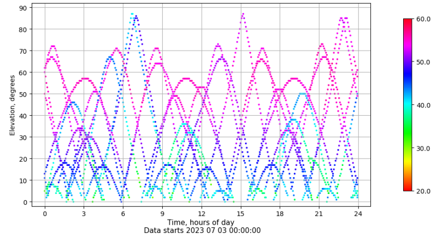
Time-elevation plot for station TALV. Signal to Noise S1C Data file TALV00ESP_R_2023184.xtr
