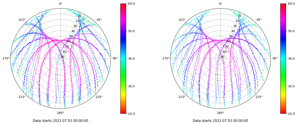
Skyplot for station TALV. Signal to Noise S1C Data file TALV00ESP_R_2023184.xtr Skyplot for station TALV. Signal to Noise S2P Data file TALV00ESP_R_2023184.xtr
