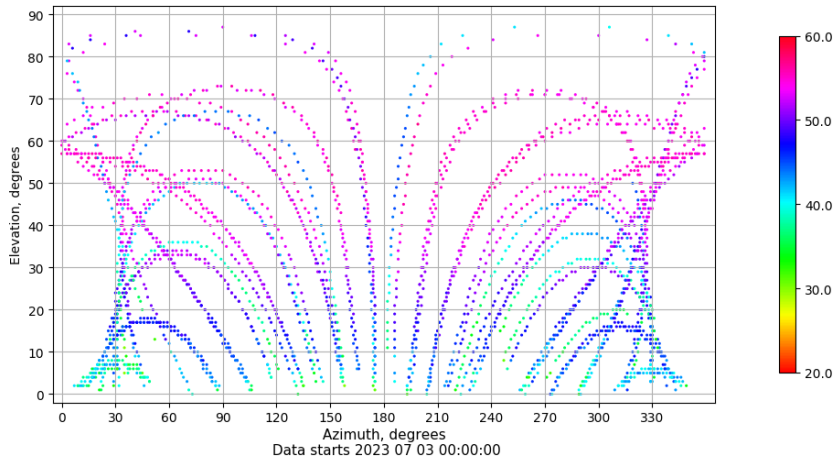
Azimuth-elevation plot for station TALV. Signal to Noise S1C Data file TALV00ESP_R_2023184.xtr
