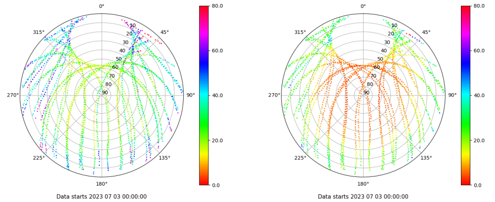
Skyplot for station TALV. Parameter M1C Data file TALV00ESP_R_2023184.xtr Skyplot for station TALV. Parameter M2P Data file TALV00ESP_R_2023184.xtr
