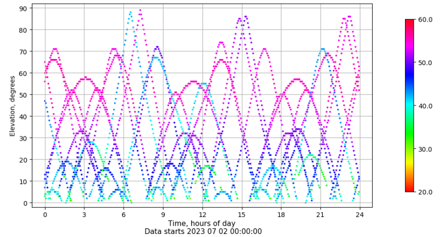
Time-elevation plot for station TALV. Signal to Noise S1C Data file TALV00ESP_R_2023183.xtr
