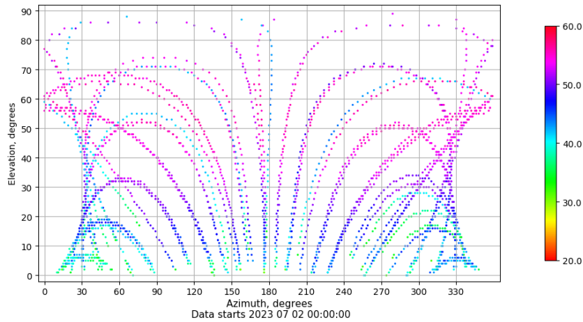
Azimuth-elevation plot for station TALV. Signal to Noise S1C Data file TALV00ESP_R_2023183.xtr
