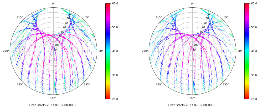
Skyplot for station TALV. Signal to Noise S1C Data file TALV00ESP_R_2023183.xtr Skyplot for station TALV. Signal to Noise S2P Data file TALV00ESP_R_2023183.xtr
