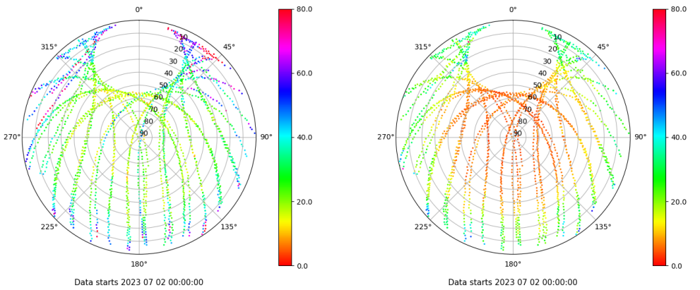
Skyplot for station TALV. Parameter M1C Data file TALV00ESP_R_2023183.xtr Skyplot for station TALV. Parameter M2P Data file TALV00ESP_R_2023183.xtr
