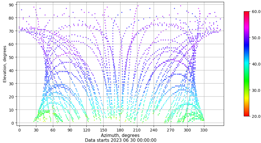
Azimuth-elevation plot for station TALV. Signal to Noise S1C Data file TALV00ESP_R_2023181.xtr
