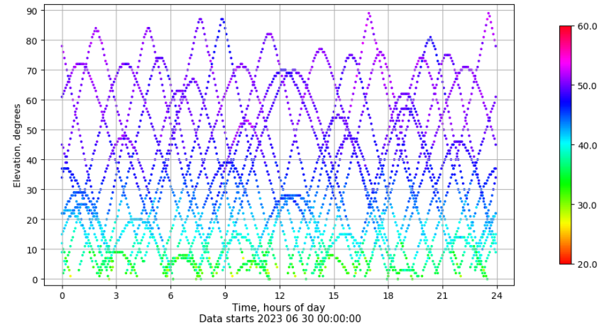
Time-elevation plot for station TALV. Signal to Noise S1C Data file TALV00ESP_R_2023181.xtr
