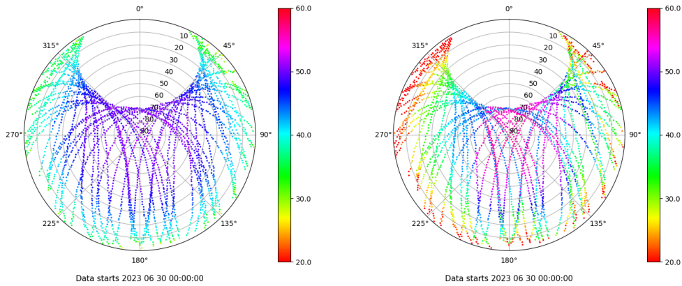
Skyplot for station TALV. Signal to Noise S1C Data file TALV00ESP_R_2023181.xtr Skyplot for station TALV. Signal to Noise S2W Data file TALV00ESP_R_2023181.xtr
