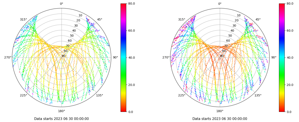
Skyplot for station TALV. Parameter M1C Data file TALV00ESP_R_2023181.xtr Skyplot for station TALV. Parameter M2W Data file TALV00ESP_R_2023181.xtr
