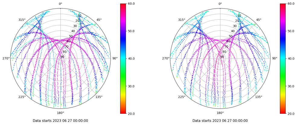
Skyplot for station TALV. Signal to Noise S1C Data file TALV00ESP_R_2023178.xtr Skyplot for station TALV. Signal to Noise S2P Data file TALV00ESP_R_2023178.xtr
