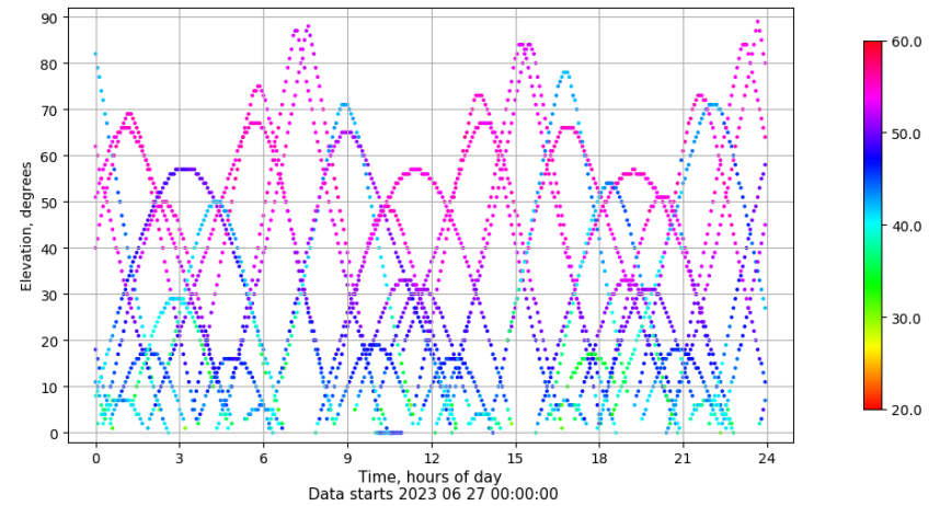
Time-elevation plot for station TALV. Signal to Noise S1C Data file TALV00ESP_R_2023178.xtr
