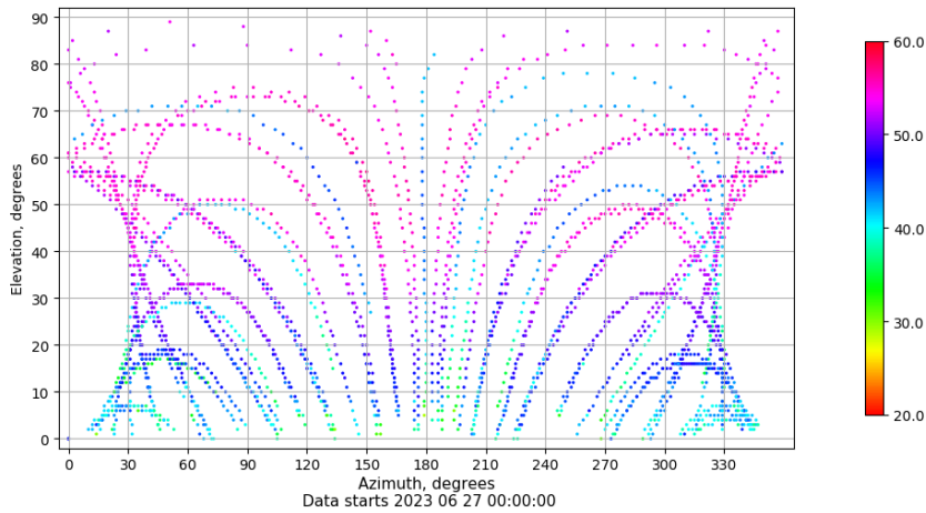
Azimuth-elevation plot for station TALV. Signal to Noise S1C Data file TALV00ESP_R_2023178.xtr
