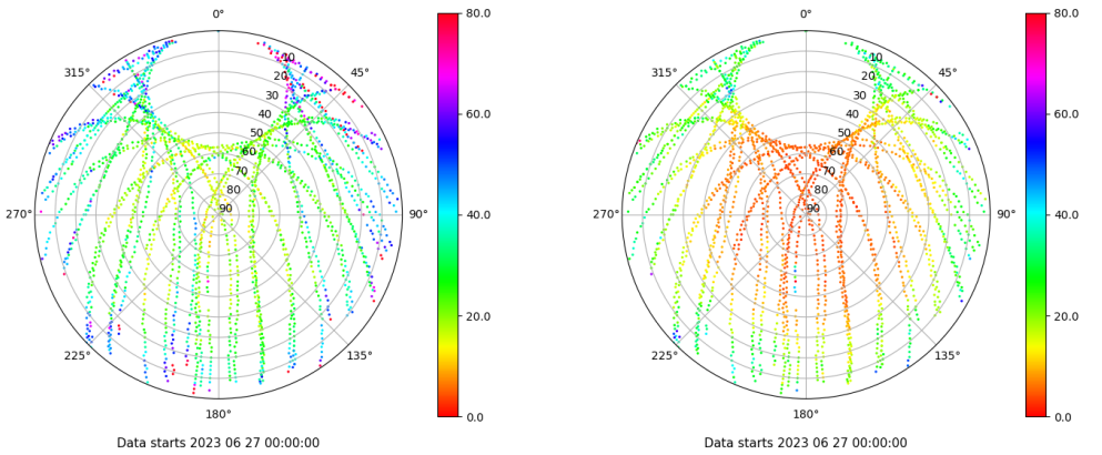
Skyplot for station TALV. Parameter M1C Data file TALV00ESP_R_2023178.xtr Skyplot for station TALV. Parameter M2P Data file TALV00ESP_R_2023178.xtr
