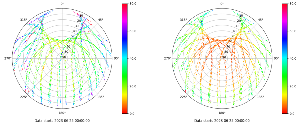
Skyplot for station TALV. Parameter M1C Data file TALV00ESP_R_2023176.xtr Skyplot for station TALV. Parameter M2P Data file TALV00ESP_R_2023176.xtr
