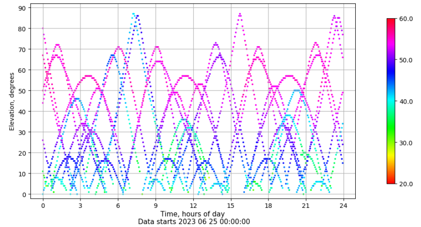
Time-elevation plot for station TALV. Signal to Noise S1C Data file TALV00ESP_R_2023176.xtr
