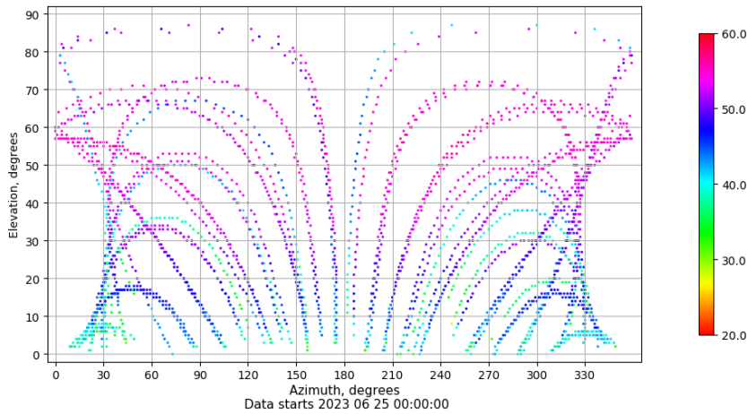
Azimuth-elevation plot for station TALV. Signal to Noise S1C Data file TALV00ESP_R_2023176.xtr
