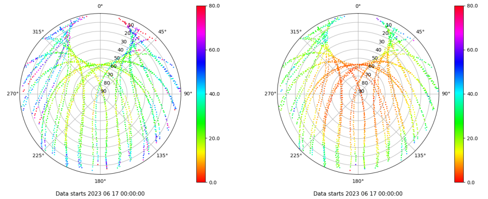
Skyplot for station TALV. Parameter M1C Data file TALV00ESP_R_2023168.xtr Skyplot for station TALV. Parameter M2P Data file TALV00ESP_R_2023168.xtr
