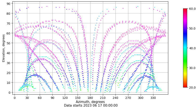
Azimuth-elevation plot for station TALV. Signal to Noise S1C Data file TALV00ESP_R_2023168.xtr
