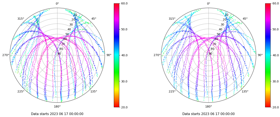
Skyplot for station TALV. Signal to Noise S1C Data file TALV00ESP_R_2023168.xtr Skyplot for station TALV. Signal to Noise S2P Data file TALV00ESP_R_2023168.xtr
