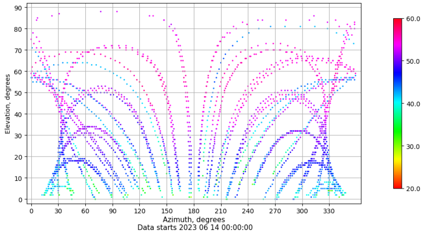
Azimuth-elevation plot for station TALV. Signal to Noise S1C Data file TALV00ESP_R_2023165.xtr
