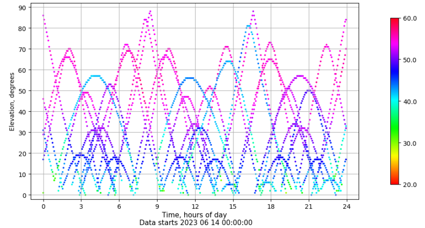
Time-elevation plot for station TALV. Signal to Noise S1C Data file TALV00ESP_R_2023165.xtr
