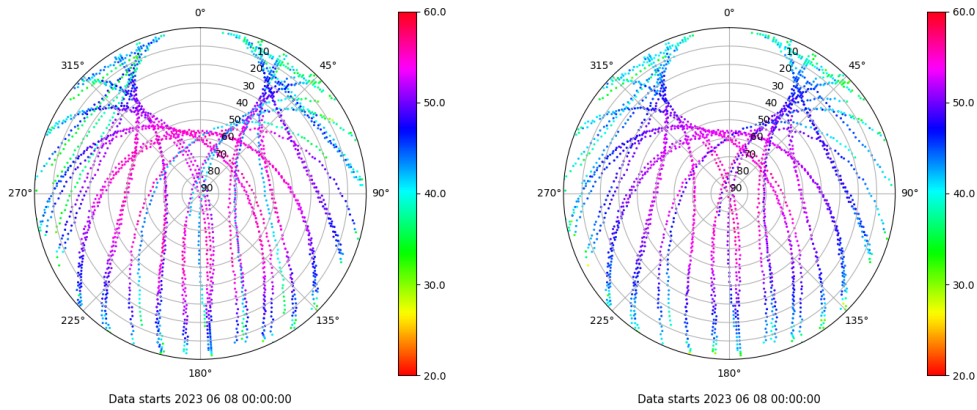
Skyplot for station TALV. Signal to Noise S1C Data file TALV00ESP_R_2023159.xtr Skyplot for station TALV. Signal to Noise S2P Data file TALV00ESP_R_2023159.xtr
