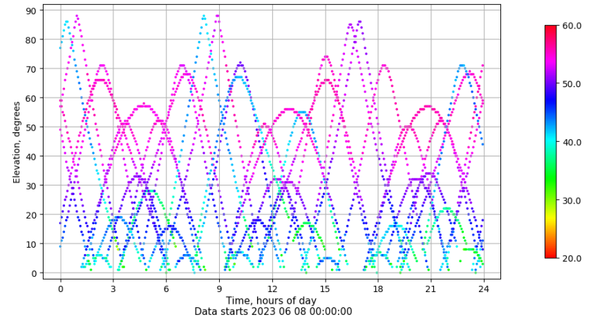
Time-elevation plot for station TALV. Signal to Noise S1C Data file TALV00ESP_R_2023159.xtr
