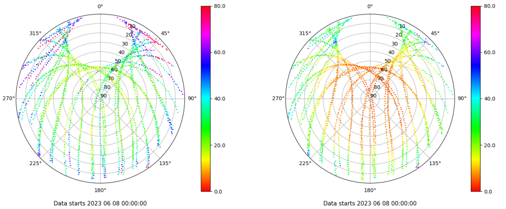
Skyplot for station TALV. Parameter M1C Data file TALV00ESP_R_2023159.xtr Skyplot for station TALV. Parameter M2P Data file TALV00ESP_R_2023159.xtr
