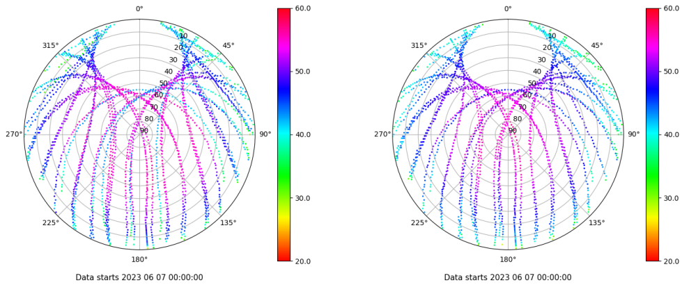
Skyplot for station TALV. Signal to Noise S1C Data file TALV00ESP_R_2023158.xtr Skyplot for station TALV. Signal to Noise S2P Data file TALV00ESP_R_2023158.xtr
