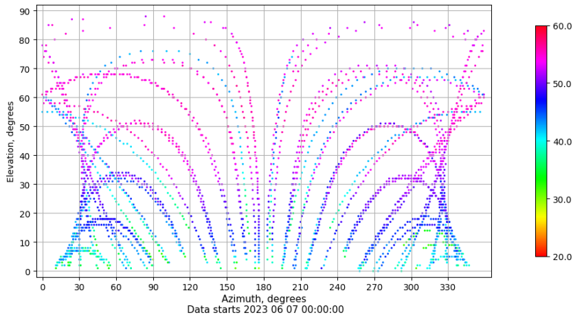
Azimuth-elevation plot for station TALV. Signal to Noise S1C Data file TALV00ESP_R_2023158.xtr
