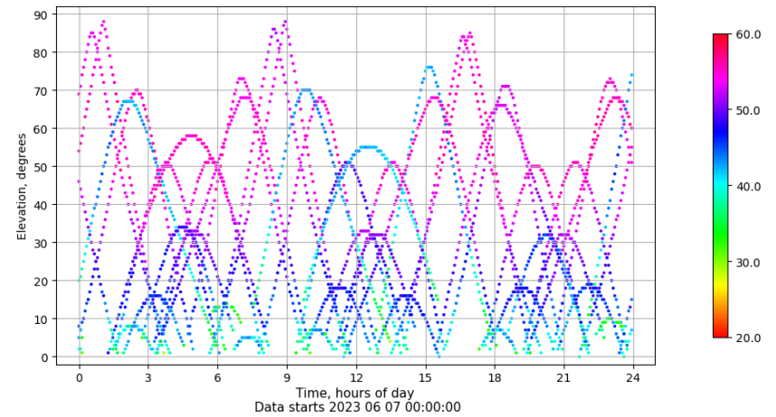
Time-elevation plot for station TALV. Signal to Noise S1C Data file TALV00ESP_R_2023158.xtr
