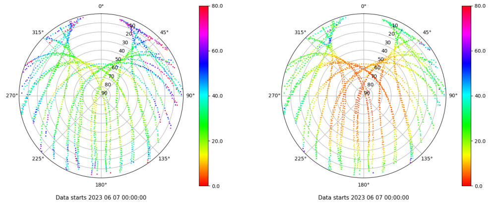
Skyplot for station TALV. Parameter M1C Data file TALV00ESP_R_2023158.xtr Skyplot for station TALV. Parameter M2P Data file TALV00ESP_R_2023158.xtr
