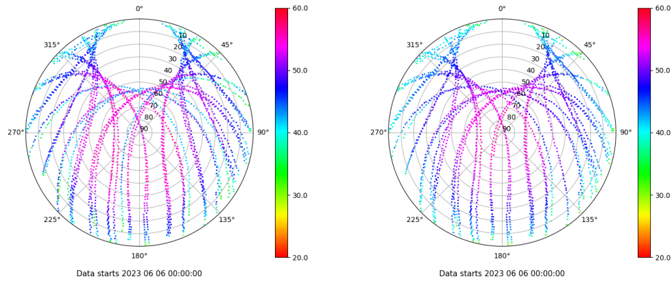
Skyplot for station TALV. Signal to Noise S1C Data file TALV00ESP_R_2023157.xtr Skyplot for station TALV. Signal to Noise S2P Data file TALV00ESP_R_2023157.xtr
