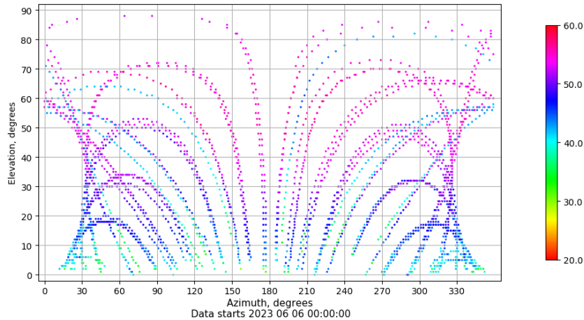
Azimuth-elevation plot for station TALV. Signal to Noise S1C Data file TALV00ESP_R_2023157.xtr
