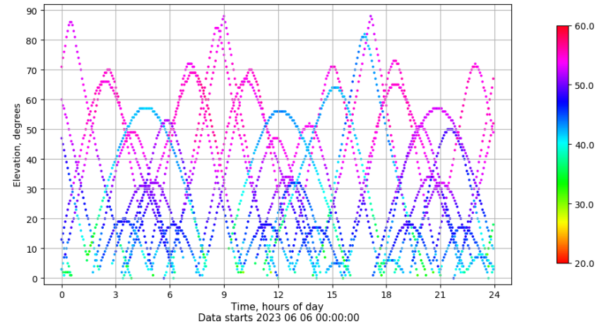
Time-elevation plot for station TALV. Signal to Noise S1C Data file TALV00ESP_R_2023157.xtr
