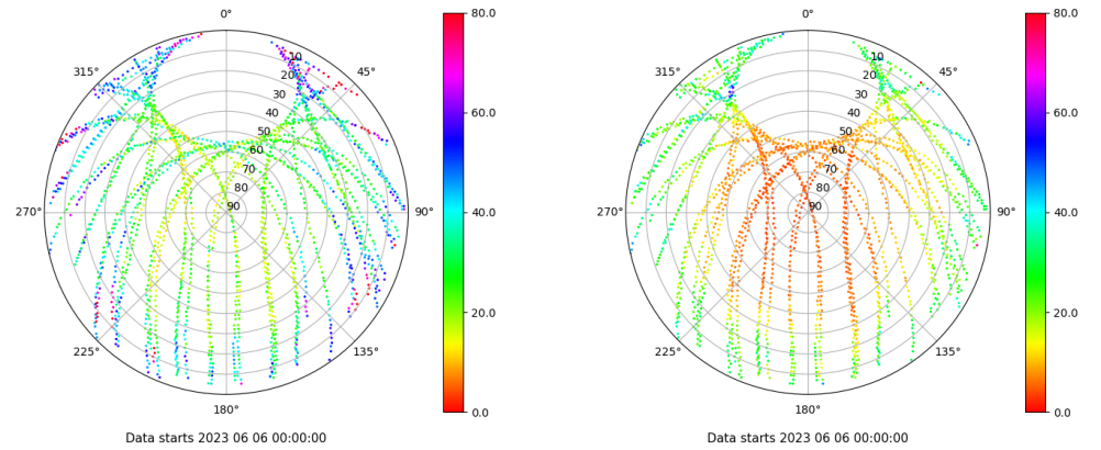
Skyplot for station TALV. Parameter M1C Data file TALV00ESP_R_2023157.xtr Skyplot for station TALV. Parameter M2P Data file TALV00ESP_R_2023157.xtr
