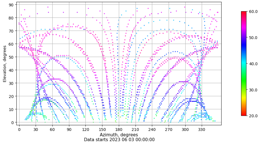
Azimuth-elevation plot for station TALV. Signal to Noise S1C Data file TALV00ESP_R_2023154.xtr
