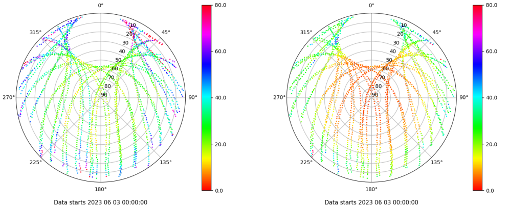
Skyplot for station TALV. Parameter M1C Data file TALV00ESP_R_2023154.xtr Skyplot for station TALV. Parameter M2P Data file TALV00ESP_R_2023154.xtr
