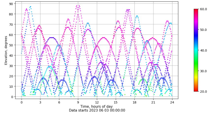
Time-elevation plot for station TALV. Signal to Noise S1C Data file TALV00ESP_R_2023154.xtr
