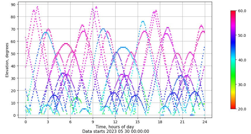
Time-elevation plot for station TALV. Signal to Noise S1C Data file TALV00ESP_R_2023150.xtr
