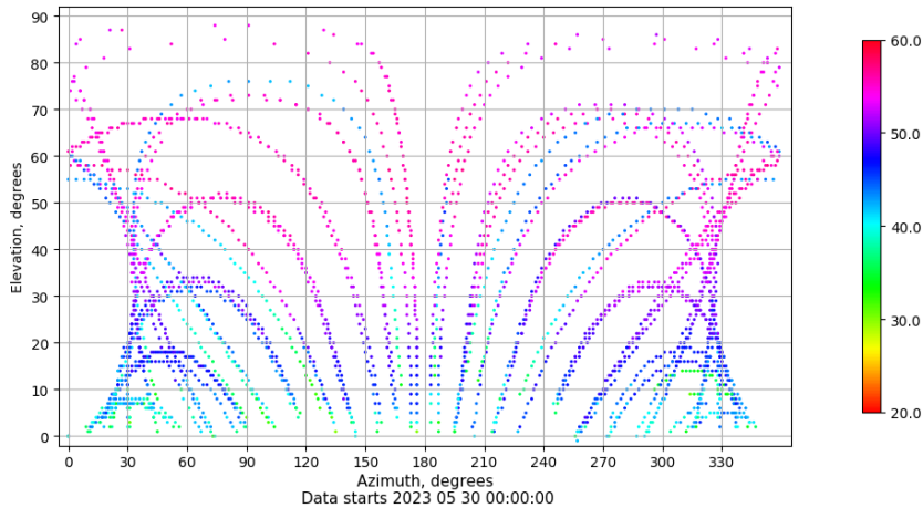
Azimuth-elevation plot for station TALV. Signal to Noise S1C Data file TALV00ESP_R_2023150.xtr
