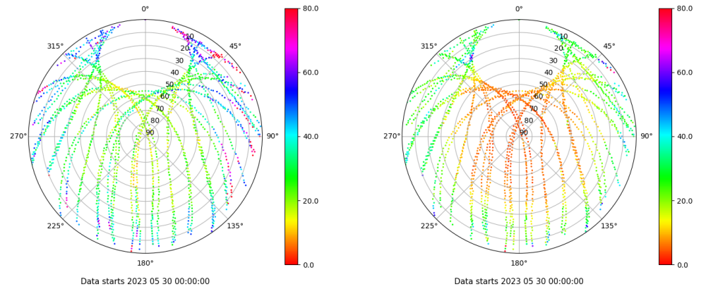
Skyplot for station TALV. Parameter M1C Data file TALV00ESP_R_2023150.xtr Skyplot for station TALV. Parameter M2P Data file TALV00ESP_R_2023150.xtr
