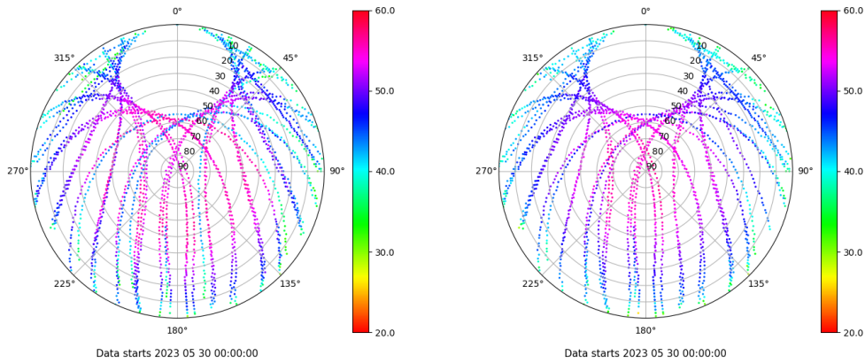
Skyplot for station TALV. Signal to Noise S1C Data file TALV00ESP_R_2023150.xtr Skyplot for station TALV. Signal to Noise S2P Data file TALV00ESP_R_2023150.xtr
