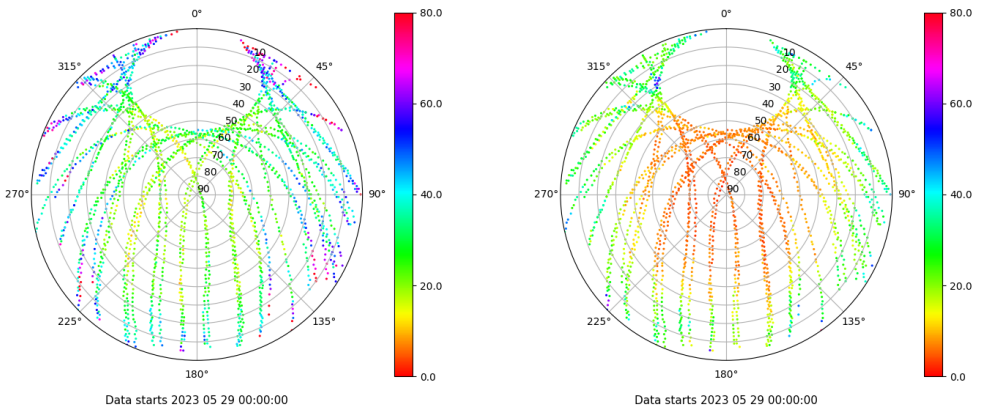
Skyplot for station TALV. Parameter M1C Data file TALV00ESP_R_2023149.xtr Skyplot for station TALV. Parameter M2P Data file TALV00ESP_R_2023149.xtr
