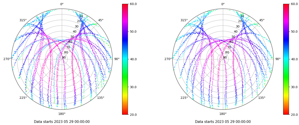
Skyplot for station TALV. Signal to Noise S1C Data file TALV00ESP_R_2023149.xtr Skyplot for station TALV. Signal to Noise S2P Data file TALV00ESP_R_2023149.xtr
