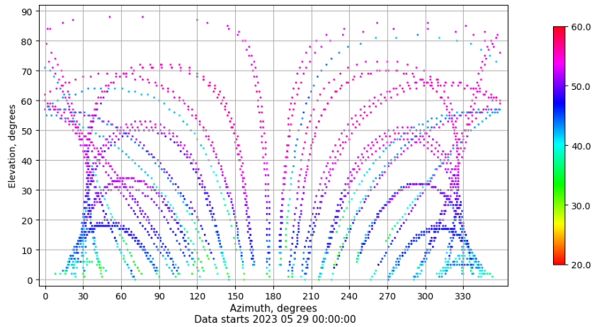
Azimuth-elevation plot for station TALV. Signal to Noise S1C Data file TALV00ESP_R_2023149.xtr
