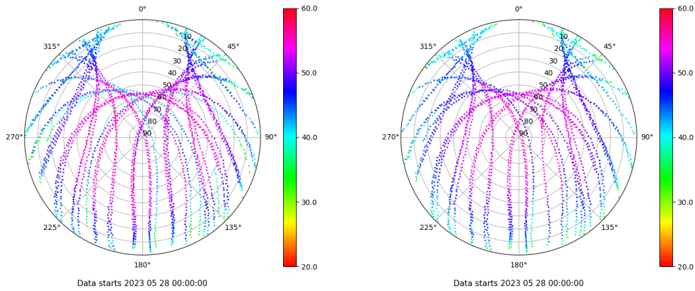
Skyplot for station TALV. Signal to Noise S1C Data file TALV00ESP_R_2023148.xtr Skyplot for station TALV. Signal to Noise S2P Data file TALV00ESP_R_2023148.xtr
