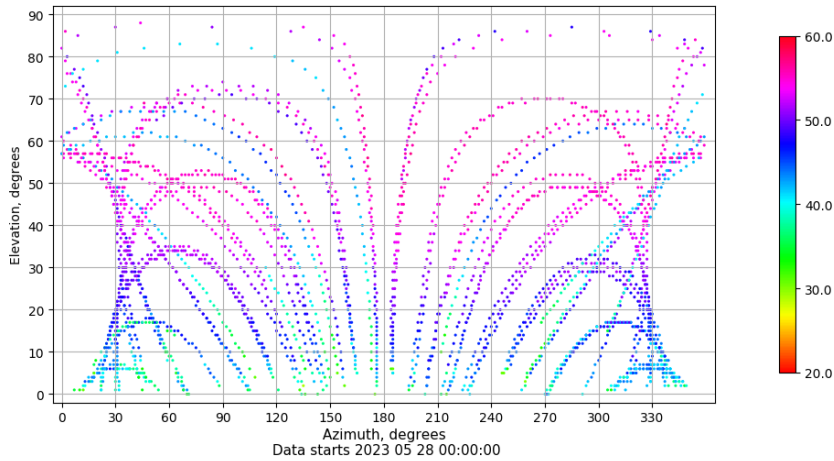
Azimuth-elevation plot for station TALV. Signal to Noise S1C Data file TALV00ESP_R_2023148.xtr
