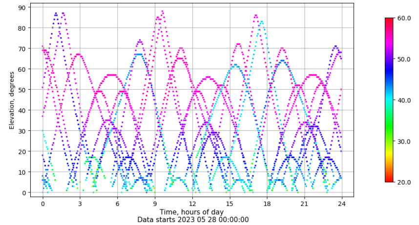
Time-elevation plot for station TALV. Signal to Noise S1C Data file TALV00ESP_R_2023148.xtr
