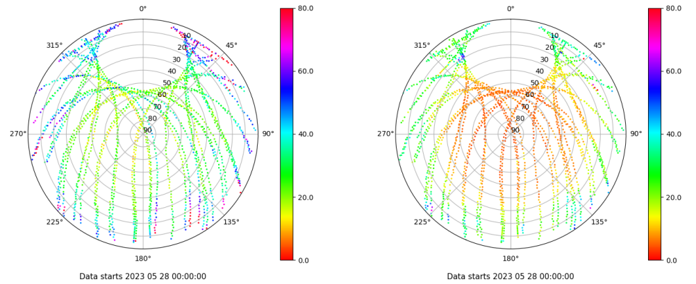
Skyplot for station TALV. Parameter M1C Data file TALV00ESP_R_2023148.xtr Skyplot for station TALV. Parameter M2P Data file TALV00ESP_R_2023148.xtr
