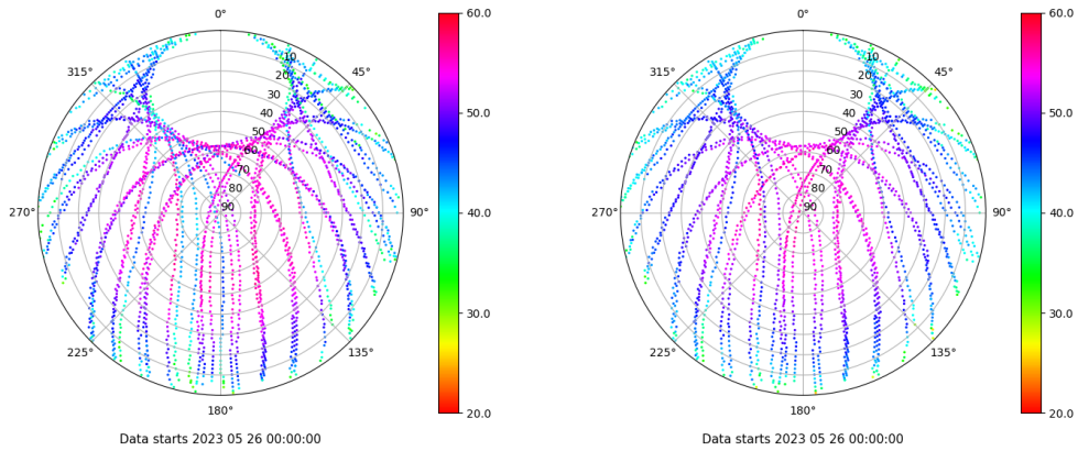
Skyplot for station TALV. Signal to Noise S1C Data file TALV00ESP_R_2023146.xtr Skyplot for station TALV. Signal to Noise S2P Data file TALV00ESP_R_2023146.xtr
