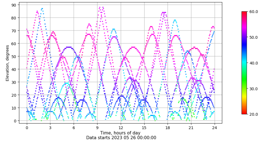
Time-elevation plot for station TALV. Signal to Noise S1C Data file TALV00ESP_R_2023146.xtr
