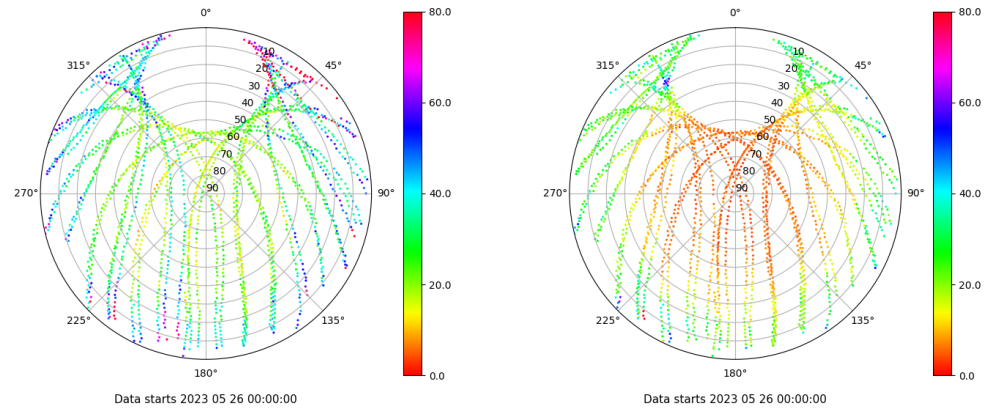
Skyplot for station TALV. Parameter M1C Data file TALV00ESP_R_2023146.xtr Skyplot for station TALV. Parameter M2P Data file TALV00ESP_R_2023146.xtr
