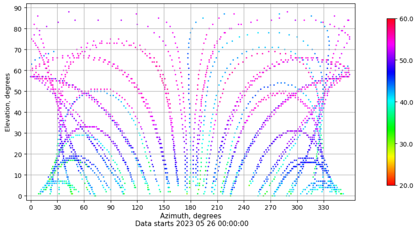
Azimuth-elevation plot for station TALV. Signal to Noise S1C Data file TALV00ESP_R_2023146.xtr
