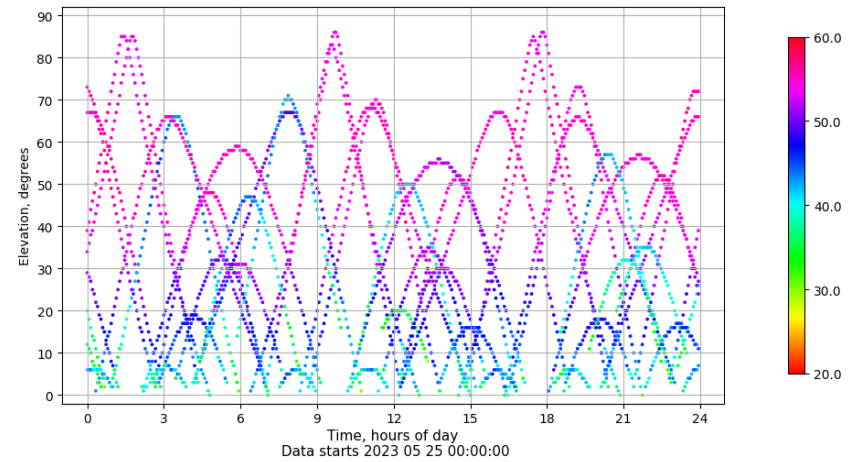
Time-elevation plot for station TALV. Signal to Noise S1C Data file TALV00ESP_R_2023145.xtr
