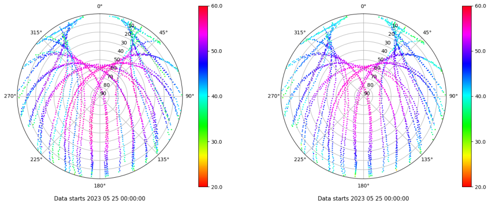
Skyplot for station TALV. Signal to Noise S1C Data file TALV00ESP_R_2023145.xtr Skyplot for station TALV. Signal to Noise S2P Data file TALV00ESP_R_2023145.xtr
