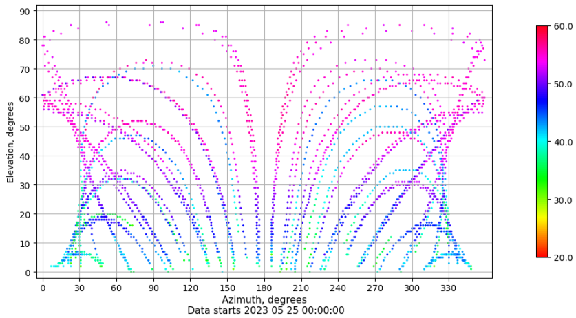
Azimuth-elevation plot for station TALV. Signal to Noise S1C Data file TALV00ESP_R_2023145.xtr
