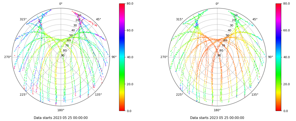
Skyplot for station TALV. Parameter M1C Data file TALV00ESP_R_2023145.xtr Skyplot for station TALV. Parameter M2P Data file TALV00ESP_R_2023145.xtr
