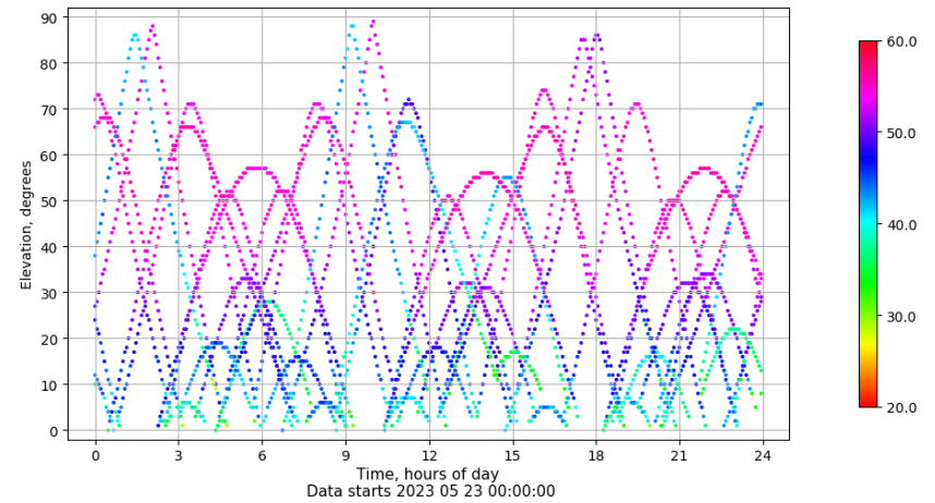
Time-elevation plot for station TALV. Signal to Noise S1C Data file TALV00ESP_R_2023143.xtr
