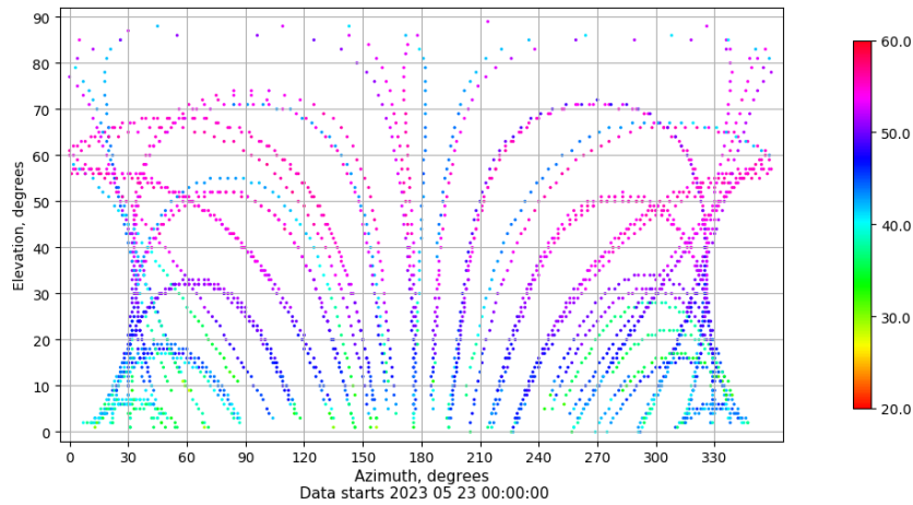
Azimuth-elevation plot for station TALV. Signal to Noise S1C Data file TALV00ESP_R_2023143.xtr
