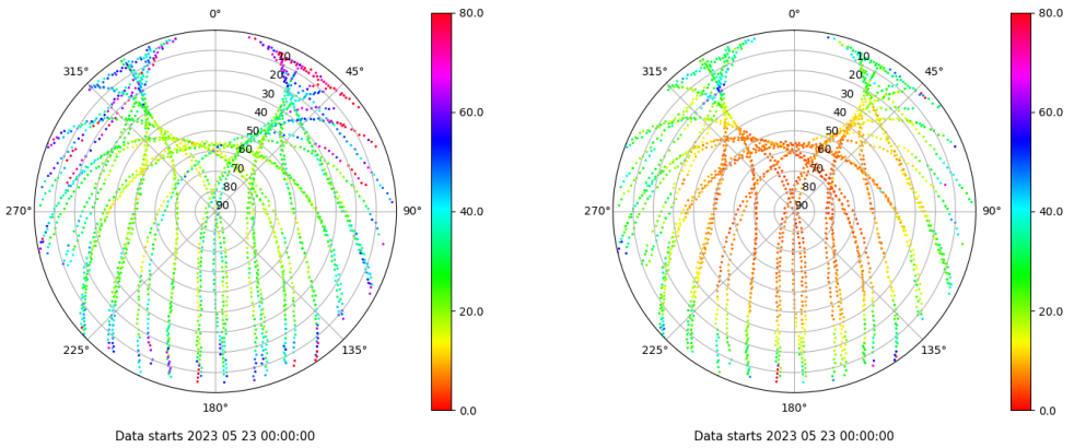
Skyplot for station TALV. Parameter M1C Data file TALV00ESP_R_2023143.xtr Skyplot for station TALV. Parameter M2P Data file TALV00ESP_R_2023143.xtr
