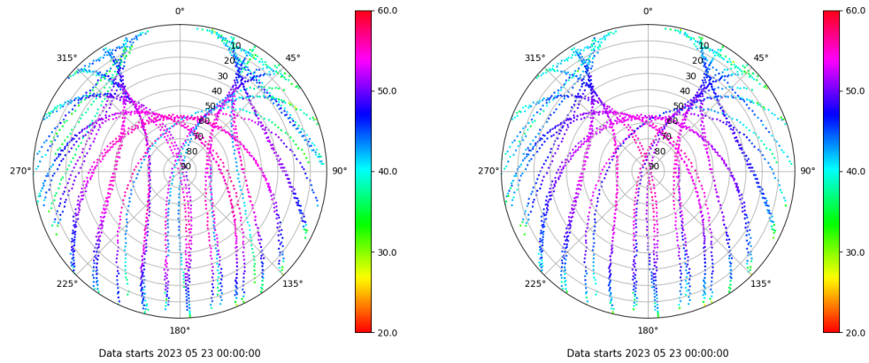
Skyplot for station TALV. Signal to Noise S1C Data file TALV00ESP_R_2023143.xtr Skyplot for station TALV. Signal to Noise S2P Data file TALV00ESP_R_2023143.xtr
