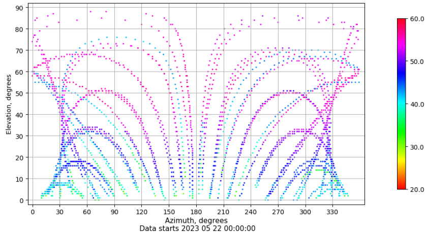
Azimuth-elevation plot for station TALV. Signal to Noise S1C Data file TALV00ESP_R_2023142.xtr
