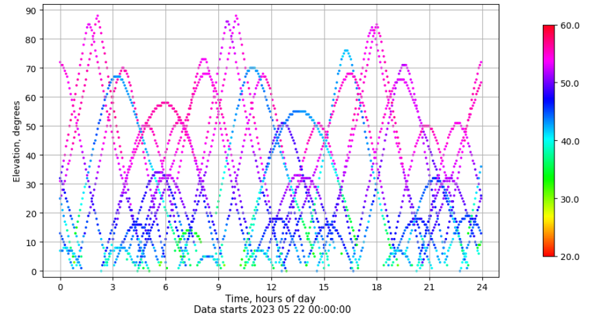
Time-elevation plot for station TALV. Signal to Noise S1C Data file TALV00ESP_R_2023142.xtr
