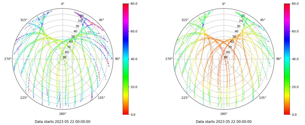
Skyplot for station TALV. Parameter M1C Data file TALV00ESP_R_2023142.xtr Skyplot for station TALV. Parameter M2P Data file TALV00ESP_R_2023142.xtr
