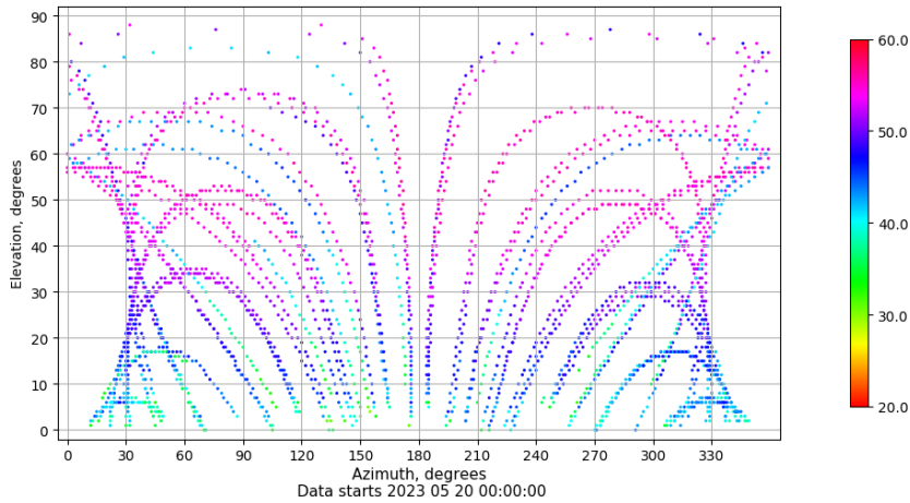
Azimuth-elevation plot for station TALV. Signal to Noise S1C Data file TALV00ESP_R_2023140.xtr
