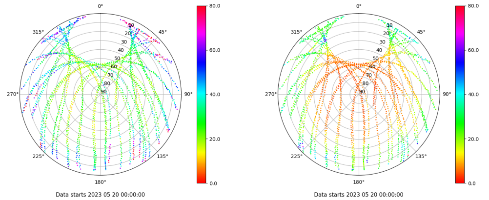
Skyplot for station TALV. Parameter M1C Data file TALV00ESP_R_2023140.xtr Skyplot for station TALV. Parameter M2P Data file TALV00ESP_R_2023140.xtr
