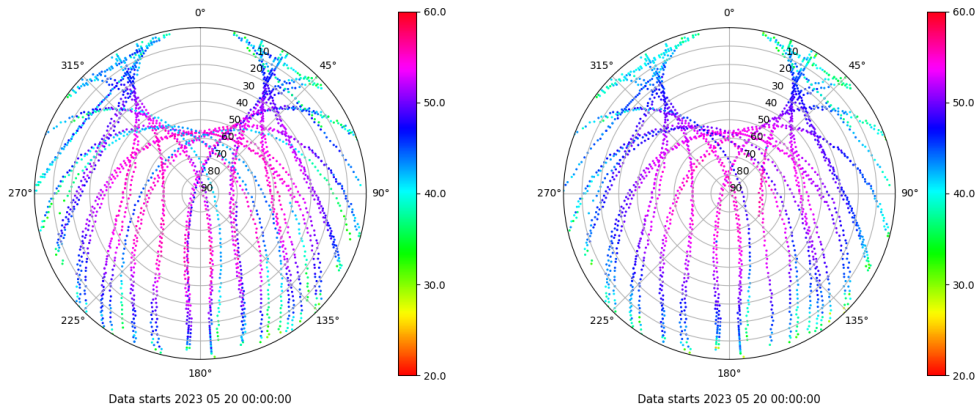
Skyplot for station TALV. Signal to Noise S1C Data file TALV00ESP_R_2023140.xtr Skyplot for station TALV. Signal to Noise S2P Data file TALV00ESP_R_2023140.xtr
