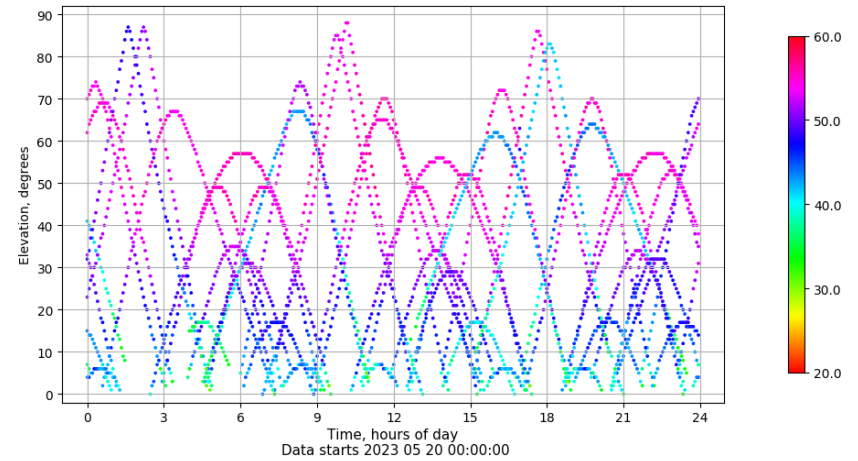
Time-elevation plot for station TALV. Signal to Noise S1C Data file TALV00ESP_R_2023140.xtr
