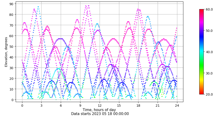
Time-elevation plot for station TALV. Signal to Noise S1C Data file TALV00ESP_R_2023138.xtr
