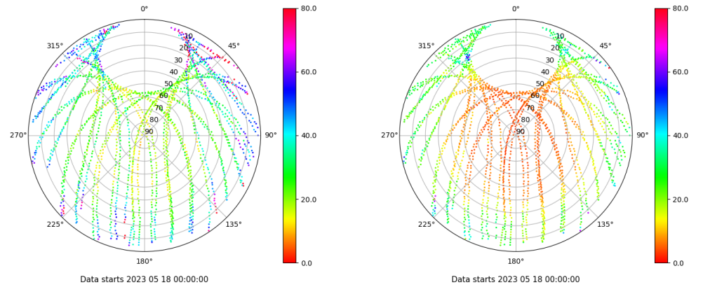
Skyplot for station TALV. Parameter M1C Data file TALV00ESP_R_2023138.xtr Skyplot for station TALV. Parameter M2P Data file TALV00ESP_R_2023138.xtr
