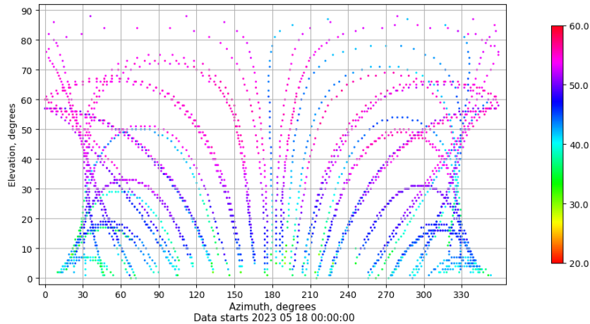
Azimuth-elevation plot for station TALV. Signal to Noise S1C Data file TALV00ESP_R_2023138.xtr
