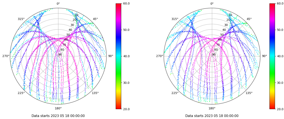
Skyplot for station TALV. Signal to Noise S1C Data file TALV00ESP_R_2023138.xtr Skyplot for station TALV. Signal to Noise S2P Data file TALV00ESP_R_2023138.xtr
