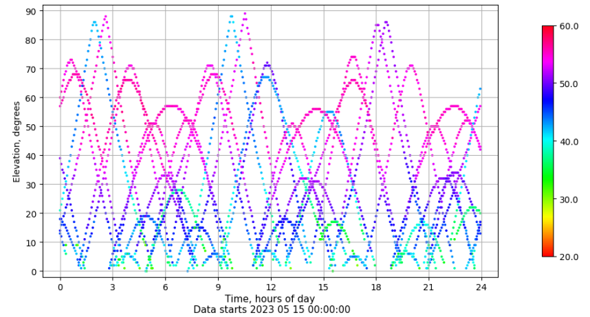
Time-elevation plot for station TALV. Signal to Noise S1C Data file TALV00ESP_R_2023135.xtr
