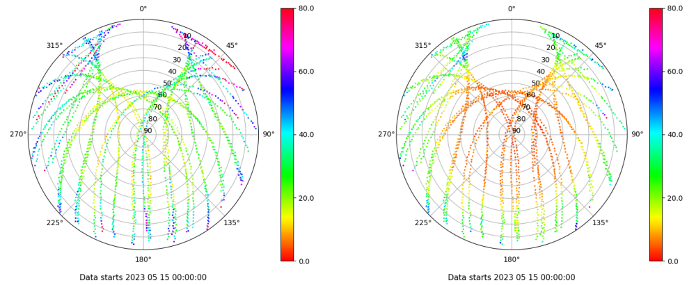
Skyplot for station TALV. Parameter M1C Data file TALV00ESP_R_2023135.xtr Skyplot for station TALV. Parameter M2P Data file TALV00ESP_R_2023135.xtr
