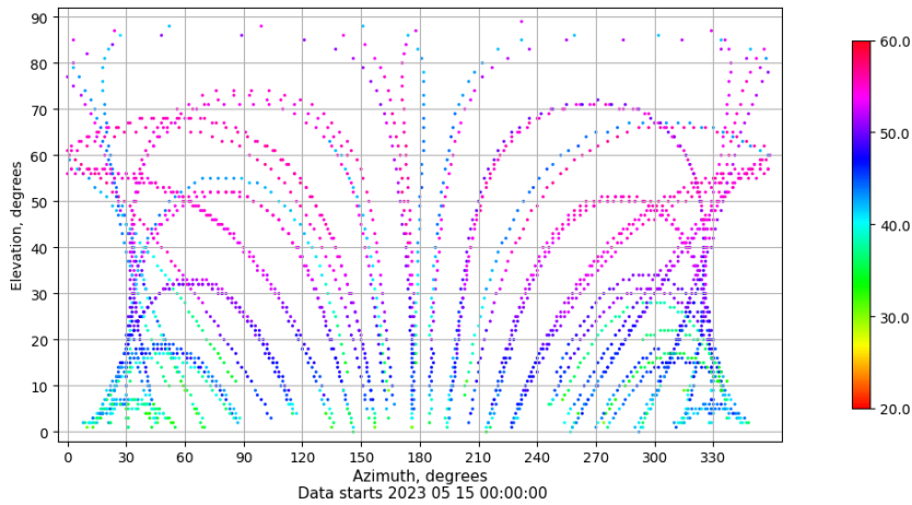
Azimuth-elevation plot for station TALV. Signal to Noise S1C Data file TALV00ESP_R_2023135.xtr
