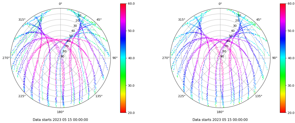
Skyplot for station TALV. Signal to Noise S1C Data file TALV00ESP_R_2023135.xtr Skyplot for station TALV. Signal to Noise S2P Data file TALV00ESP_R_2023135.xtr
