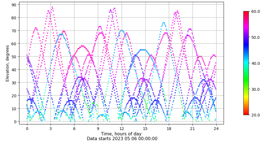
Time-elevation plot for station TALV. Signal to Noise S1C Data file TALV00ESP_R_2023126.xtr
