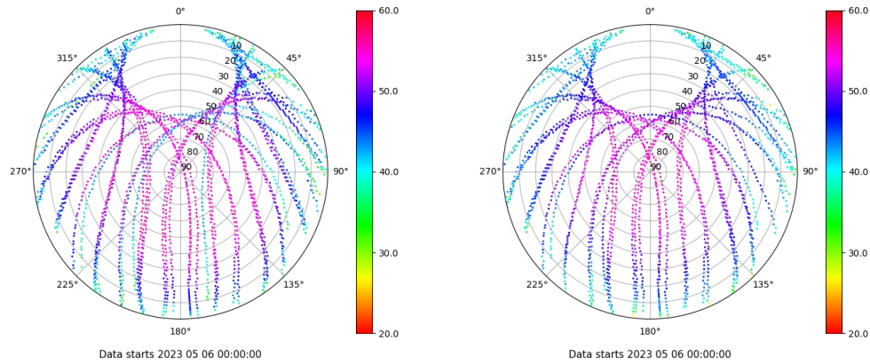
Skyplot for station TALV. Signal to Noise S1C Data file TALV00ESP_R_2023126.xtr Skyplot for station TALV. Signal to Noise S2P Data file TALV00ESP_R_2023126.xtr
