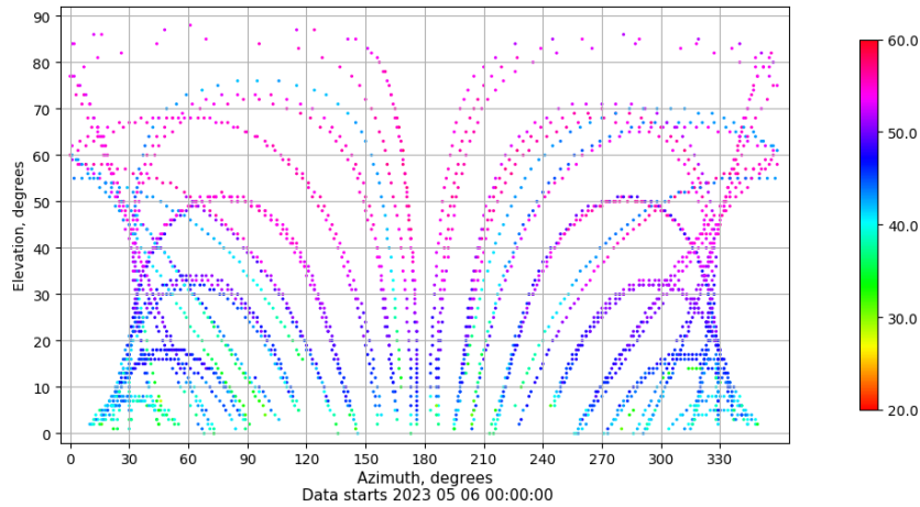
Azimuth-elevation plot for station TALV. Signal to Noise S1C Data file TALV00ESP_R_2023126.xtr
