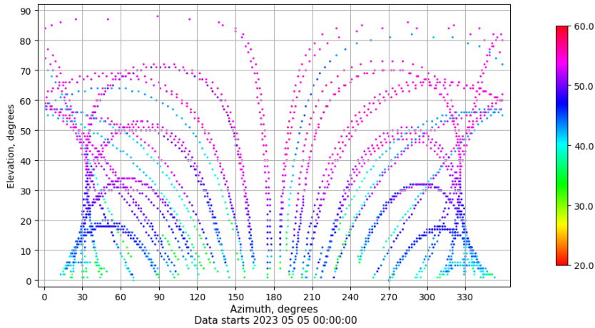
Azimuth-elevation plot for station TALV. Signal to Noise S1C Data file TALV00ESP_R_2023125.xtr
