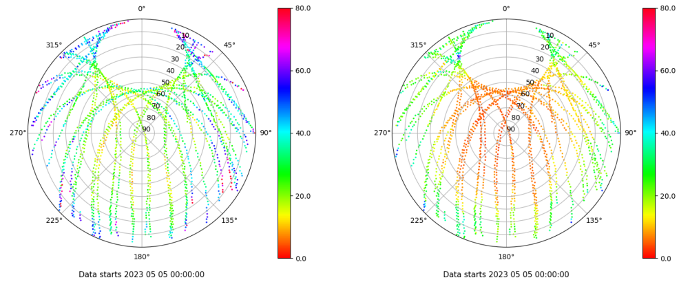
Skyplot for station TALV. Parameter M1C Data file TALV00ESP_R_2023125.xtr Skyplot for station TALV. Parameter M2P Data file TALV00ESP_R_2023125.xtr
