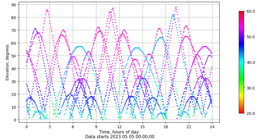
Time-elevation plot for station TALV. Signal to Noise S1C Data file TALV00ESP_R_2023125.xtr
