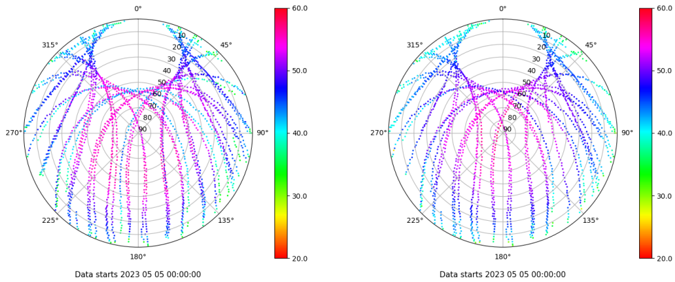
Skyplot for station TALV. Signal to Noise S1C Data file TALV00ESP_R_2023125.xtr Skyplot for station TALV. Signal to Noise S2P Data file TALV00ESP_R_2023125.xtr
