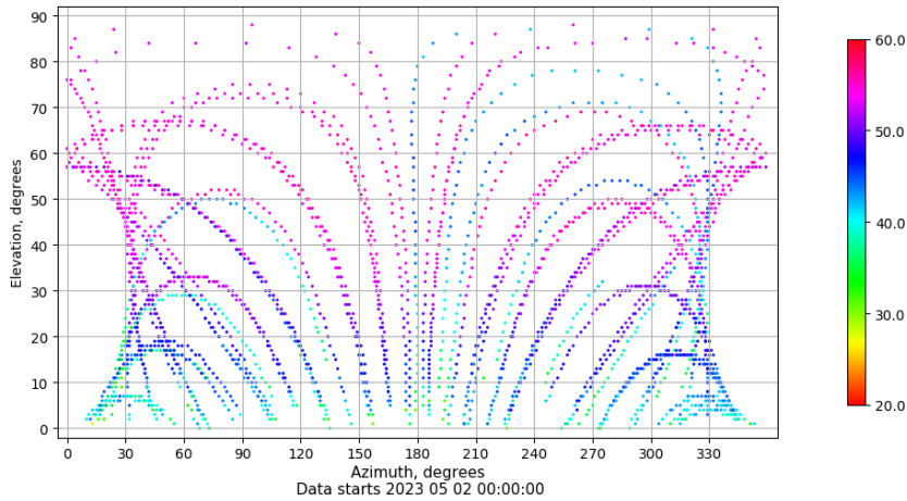
Azimuth-elevation plot for station TALV. Signal to Noise S1C Data file TALV00ESP_R_2023122.xtr
