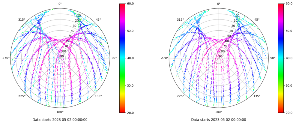
Skyplot for station TALV. Signal to Noise S1C Data file TALV00ESP_R_2023122.xtr Skyplot for station TALV. Signal to Noise S2P Data file TALV00ESP_R_2023122.xtr
