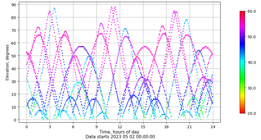
Time-elevation plot for station TALV. Signal to Noise S1C Data file TALV00ESP_R_2023122.xtr
