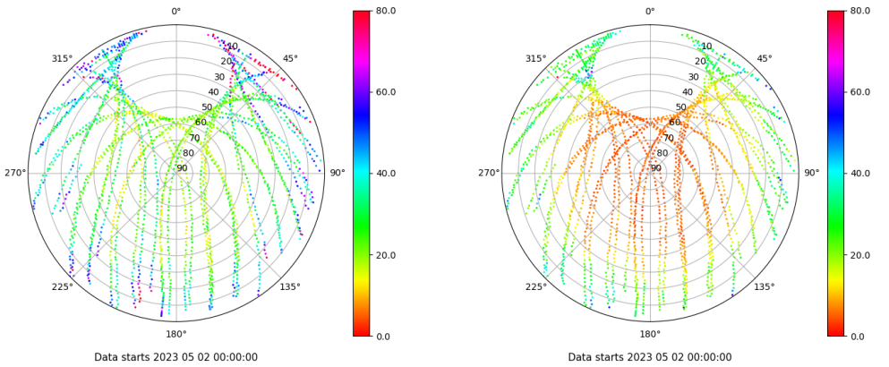
Skyplot for station TALV. Parameter M1C Data file TALV00ESP_R_2023122.xtr Skyplot for station TALV. Parameter M2P Data file TALV00ESP_R_2023122.xtr
