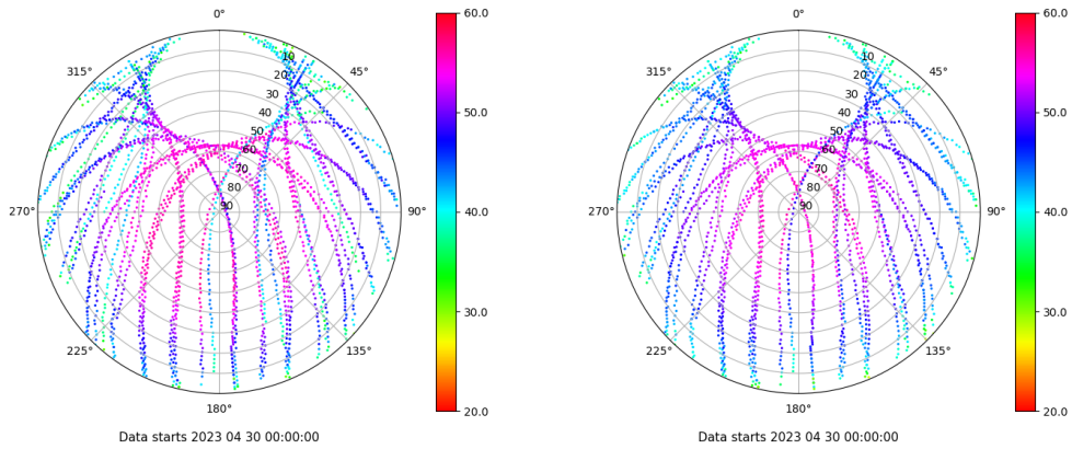
Skyplot for station TALV. Signal to Noise S1C Data file TALV00ESP_R_2023120.xtr Skyplot for station TALV. Signal to Noise S2P Data file TALV00ESP_R_2023120.xtr
