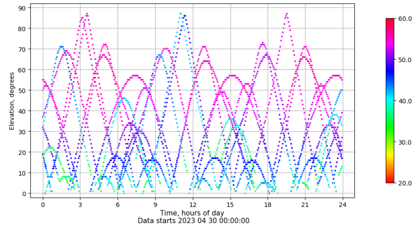
Time-elevation plot for station TALV. Signal to Noise S1C Data file TALV00ESP_R_2023120.xtr
