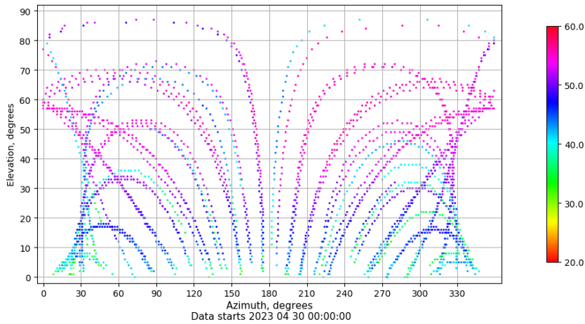
Azimuth-elevation plot for station TALV. Signal to Noise S1C Data file TALV00ESP_R_2023120.xtr
