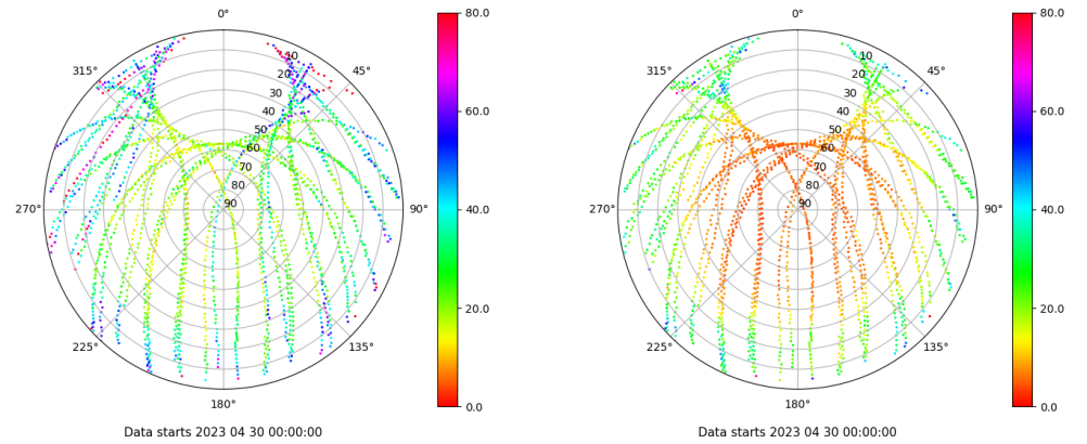
Skyplot for station TALV. Parameter M1C Data file TALV00ESP_R_2023120.xtr Skyplot for station TALV. Parameter M2P Data file TALV00ESP_R_2023120.xtr
