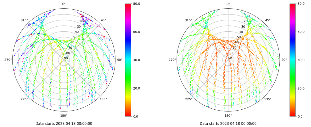
Skyplot for station TALV. Parameter M1C Data file TALV00ESP_R_2023108.xtr Skyplot for station TALV. Parameter M2P Data file TALV00ESP_R_2023108.xtr
