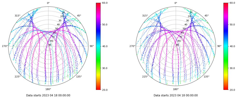
Skyplot for station TALV. Signal to Noise S1C Data file TALV00ESP_R_2023108.xtr Skyplot for station TALV. Signal to Noise S2P Data file TALV00ESP_R_2023108.xtr
