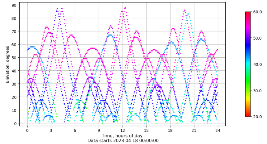
Time-elevation plot for station TALV. Signal to Noise S1C Data file TALV00ESP_R_2023108.xtr
