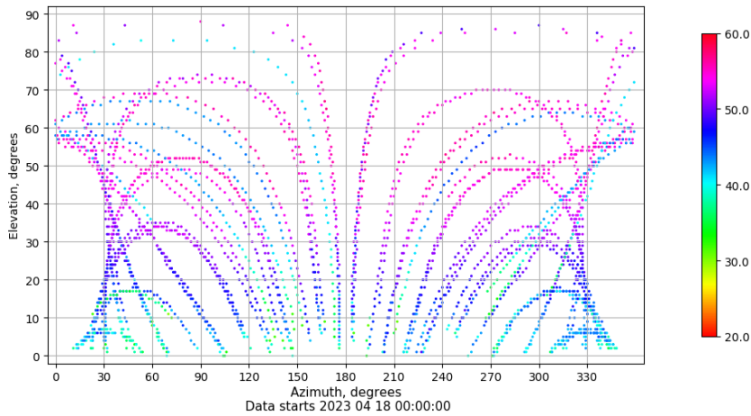
Azimuth-elevation plot for station TALV. Signal to Noise S1C Data file TALV00ESP_R_2023108.xtr
