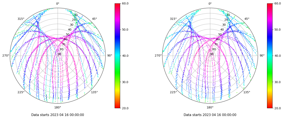
Skyplot for station TALV. Signal to Noise S1C Data file TALV00ESP_R_2023106.xtr Skyplot for station TALV. Signal to Noise S2P Data file TALV00ESP_R_2023106.xtr
