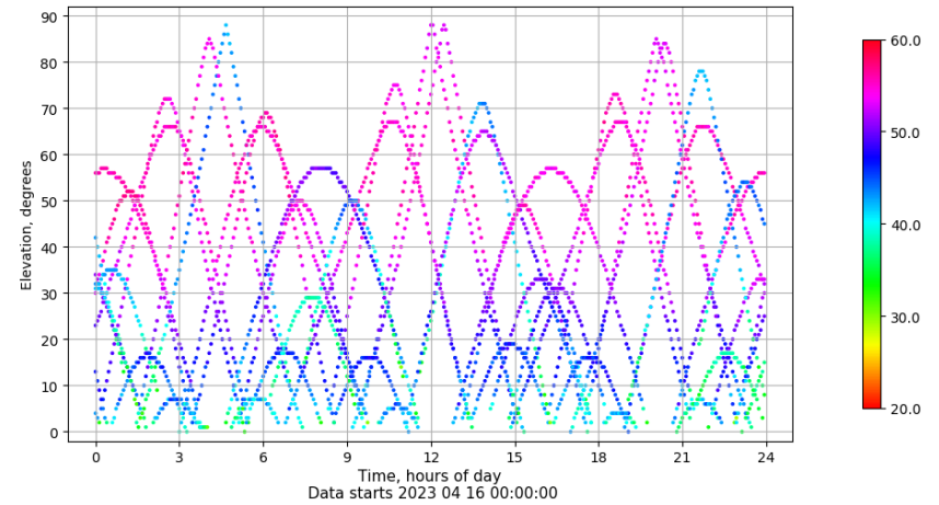
Time-elevation plot for station TALV. Signal to Noise S1C Data file TALV00ESP_R_2023106.xtr
