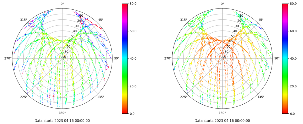
Skyplot for station TALV. Parameter M1C Data file TALV00ESP_R_2023106.xtr Skyplot for station TALV. Parameter M2P Data file TALV00ESP_R_2023106.xtr
