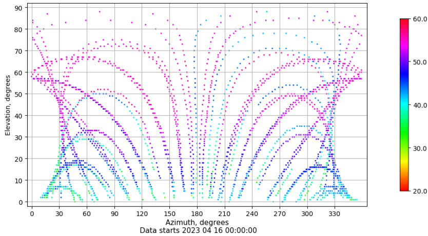
Azimuth-elevation plot for station TALV. Signal to Noise S1C Data file TALV00ESP_R_2023106.xtr
