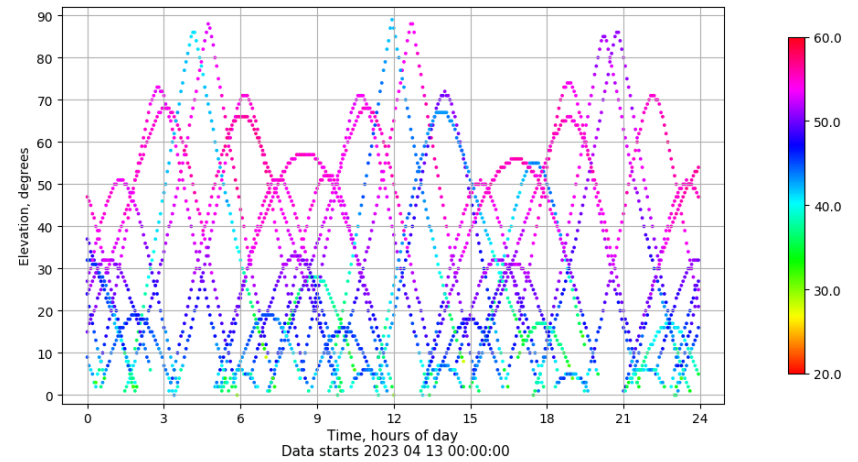
Time-elevation plot for station TALV. Signal to Noise S1C Data file TALV00ESP_R_2023103.xtr
