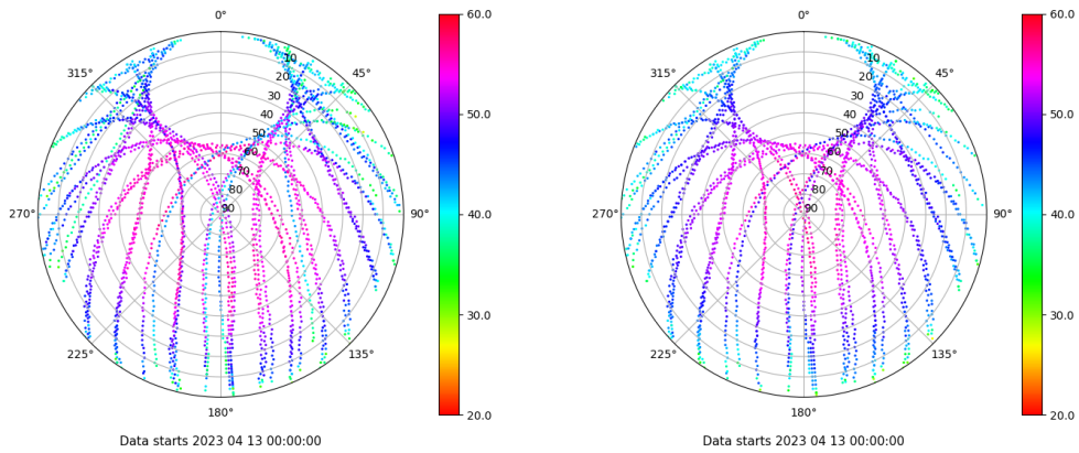
Skyplot for station TALV. Signal to Noise S1C Data file TALV00ESP_R_2023103.xtr Skyplot for station TALV. Signal to Noise S2P Data file TALV00ESP_R_2023103.xtr
