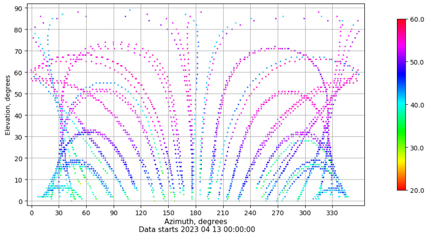
Azimuth-elevation plot for station TALV. Signal to Noise S1C Data file TALV00ESP_R_2023103.xtr
