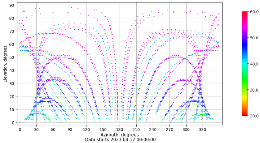
Azimuth-elevation plot for station TALV. Signal to Noise S1C Data file TALV00ESP_R_2023102.xtr
