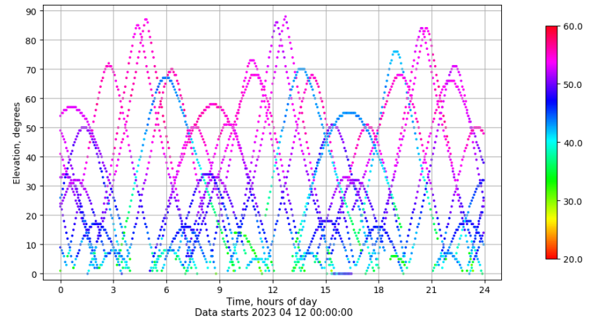
Time-elevation plot for station TALV. Signal to Noise S1C Data file TALV00ESP_R_2023102.xtr
