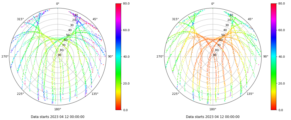
Skyplot for station TALV. Parameter M1C Data file TALV00ESP_R_2023102.xtr Skyplot for station TALV. Parameter M2P Data file TALV00ESP_R_2023102.xtr
