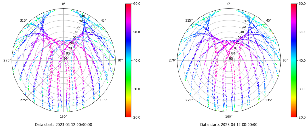
Skyplot for station TALV. Signal to Noise S1C Data file TALV00ESP_R_2023102.xtr Skyplot for station TALV. Signal to Noise S2P Data file TALV00ESP_R_2023102.xtr
