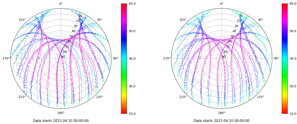
Skyplot for station TALV. Signal to Noise S1C Data file TALV00ESP_R_2023100.xtr Skyplot for station TALV. Signal to Noise S2P Data file TALV00ESP_R_2023100.xtr
