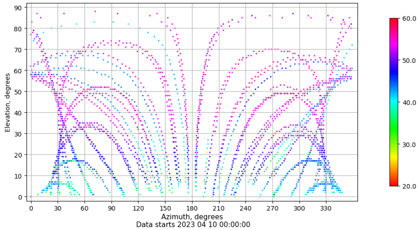
Azimuth-elevation plot for station TALV. Signal to Noise S1C Data file TALV00ESP_R_2023100.xtr
