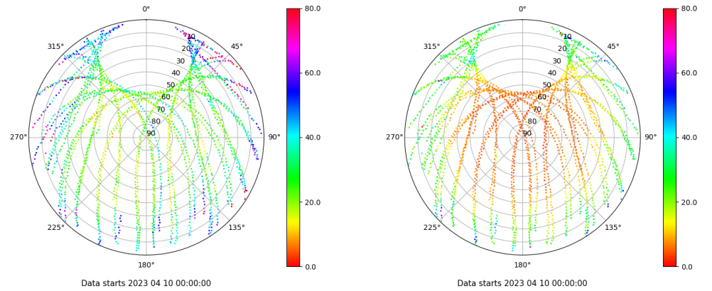
Skyplot for station TALV. Parameter M1C Data file TALV00ESP_R_2023100.xtr Skyplot for station TALV. Parameter M2P Data file TALV00ESP_R_2023100.xtr
