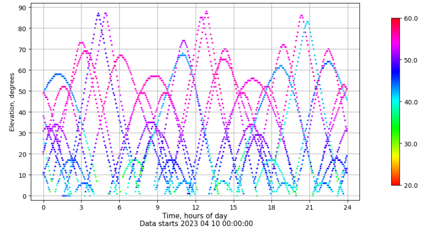
Time-elevation plot for station TALV. Signal to Noise S1C Data file TALV00ESP_R_2023100.xtr
