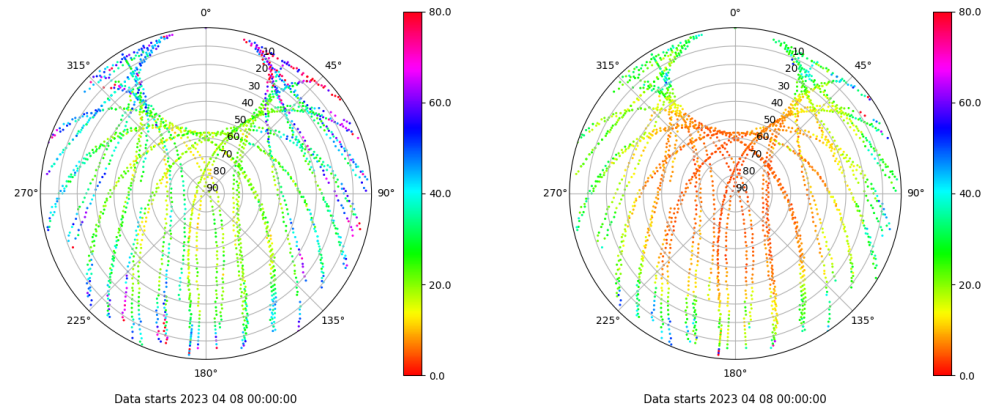
Skyplot for station TALV. Parameter M1C Data file TALV00ESP_R_2023098.xtr Skyplot for station TALV. Parameter M2P Data file TALV00ESP_R_2023098.xtr
