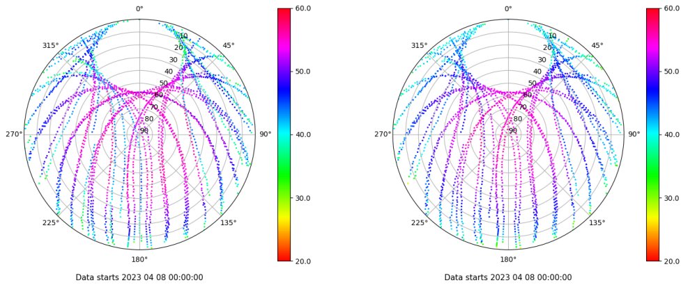
Skyplot for station TALV. Signal to Noise S1C Data file TALV00ESP_R_2023098.xtr Skyplot for station TALV. Signal to Noise S2P Data file TALV00ESP_R_2023098.xtr
