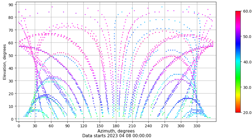
Azimuth-elevation plot for station TALV. Signal to Noise S1C Data file TALV00ESP_R_2023098.xtr
