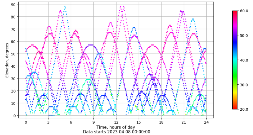
Time-elevation plot for station TALV. Signal to Noise S1C Data file TALV00ESP_R_2023098.xtr
