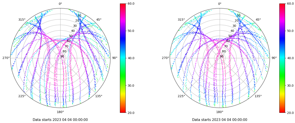
Skyplot for station TALV. Signal to Noise S1C Data file TALV00ESP_R_2023094.xtr Skyplot for station TALV. Signal to Noise S2P Data file TALV00ESP_R_2023094.xtr
