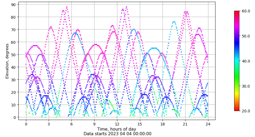
Time-elevation plot for station TALV. Signal to Noise S1C Data file TALV00ESP_R_2023094.xtr
