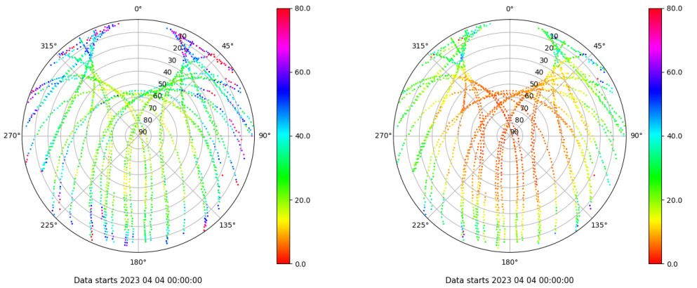
Skyplot for station TALV. Parameter M1C Data file TALV00ESP_R_2023094.xtr Skyplot for station TALV. Parameter M2P Data file TALV00ESP_R_2023094.xtr
