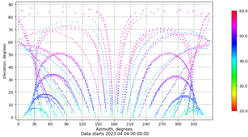
Azimuth-elevation plot for station TALV. Signal to Noise S1C Data file TALV00ESP_R_2023094.xtr
