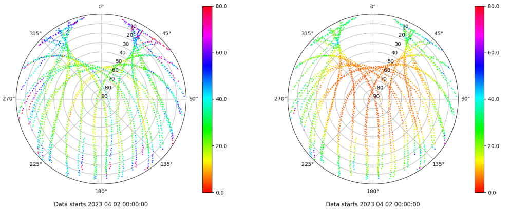
Skyplot for station TALV. Parameter M1C Data file TALV00ESP_R_2023092.xtr Skyplot for station TALV. Parameter M2P Data file TALV00ESP_R_2023092.xtr
