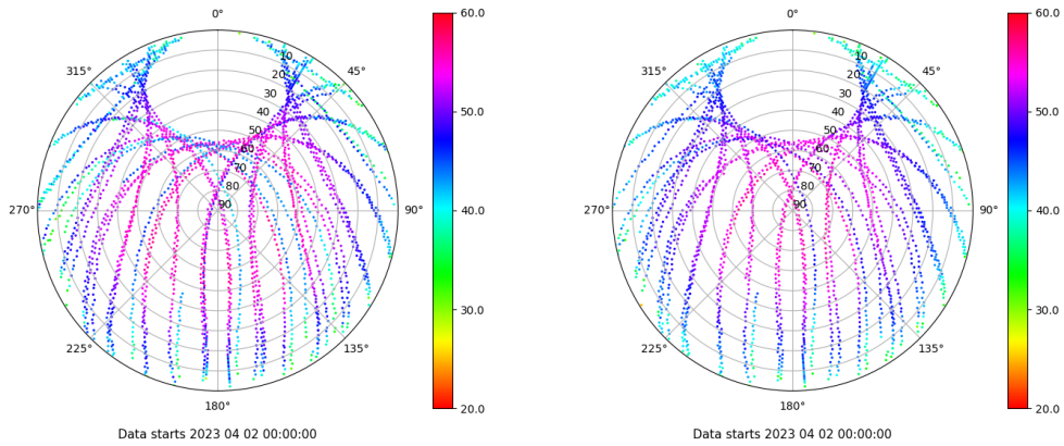
Skyplot for station TALV. Signal to Noise S1C Data file TALV00ESP_R_2023092.xtr Skyplot for station TALV. Signal to Noise S2P Data file TALV00ESP_R_2023092.xtr
