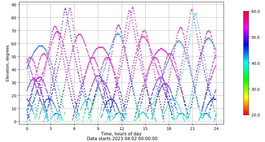
Time-elevation plot for station TALV. Signal to Noise S1C Data file TALV00ESP_R_2023092.xtr
