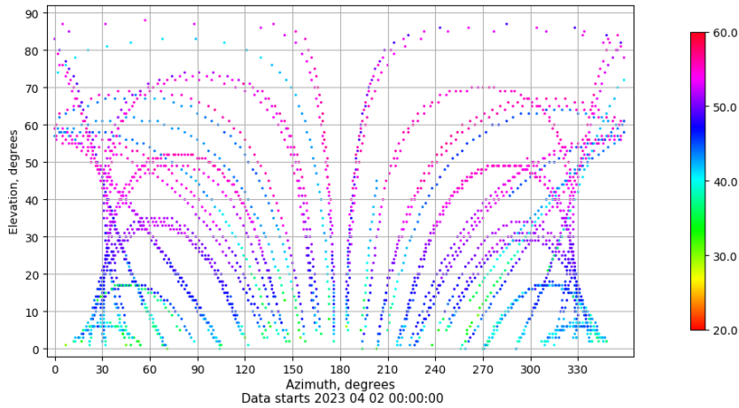
Azimuth-elevation plot for station TALV. Signal to Noise S1C Data file TALV00ESP_R_2023092.xtr
