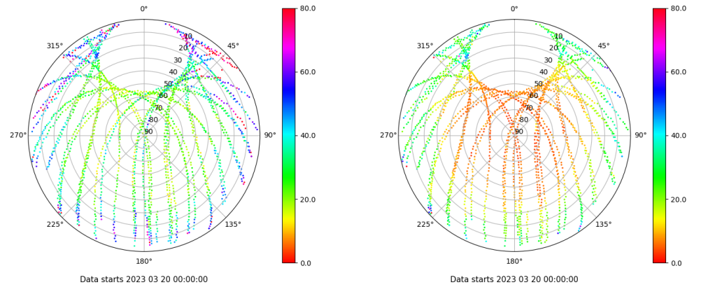
Skyplot for station TALV. Parameter M1C Data file TALV00ESP_R_2023079.xtr Skyplot for station TALV. Parameter M2P Data file TALV00ESP_R_2023079.xtr
