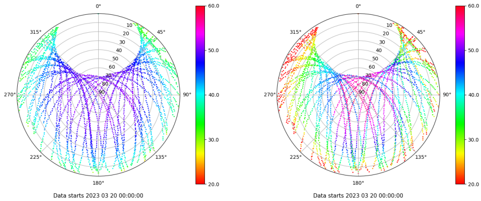
Skyplot for station TALV. Signal to Noise S1C Data file TALV00ESP_R_2023079.xtr Skyplot for station TALV. Signal to Noise S2W Data file TALV00ESP_R_2023079.xtr
