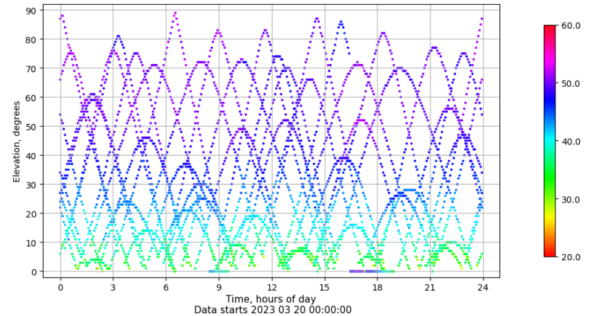
Time-elevation plot for station TALV. Signal to Noise S1C Data file TALV00ESP_R_2023079.xtr
