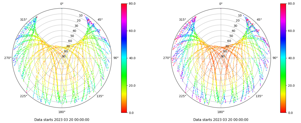
Skyplot for station TALV. Parameter M1C Data file TALV00ESP_R_2023079.xtr Skyplot for station TALV. Parameter M2W Data file TALV00ESP_R_2023079.xtr
