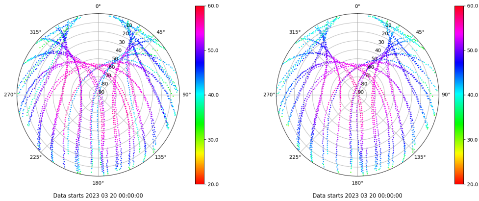
Skyplot for station TALV. Signal to Noise S1C Data file TALV00ESP_R_2023079.xtr Skyplot for station TALV. Signal to Noise S2P Data file TALV00ESP_R_2023079.xtr
