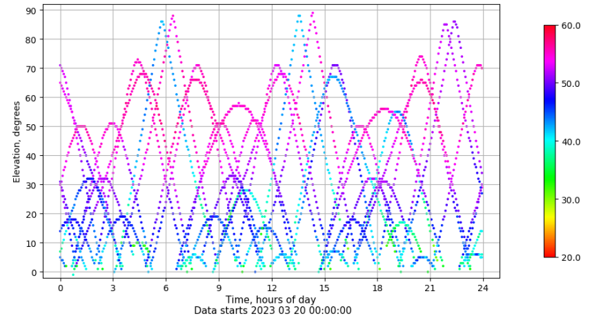
Time-elevation plot for station TALV. Signal to Noise S1C Data file TALV00ESP_R_2023079.xtr
