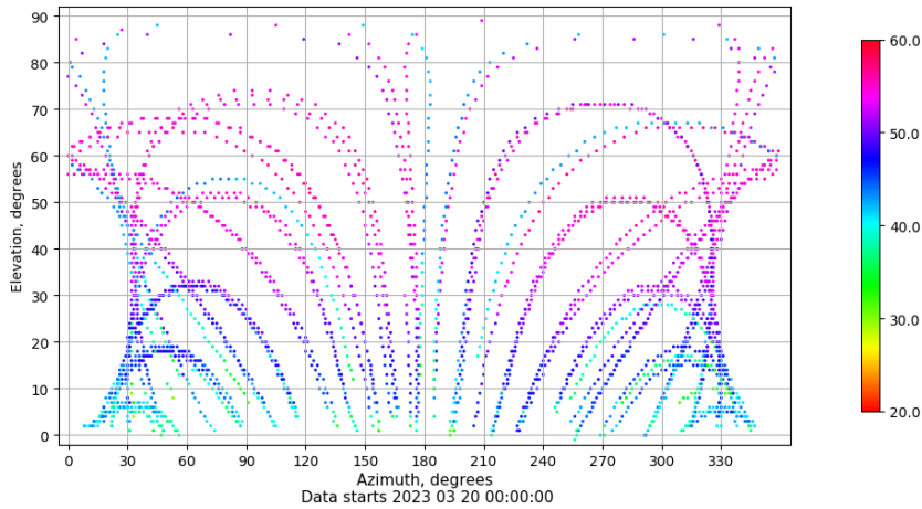
Azimuth-elevation plot for station TALV. Signal to Noise S1C Data file TALV00ESP_R_2023079.xtr
